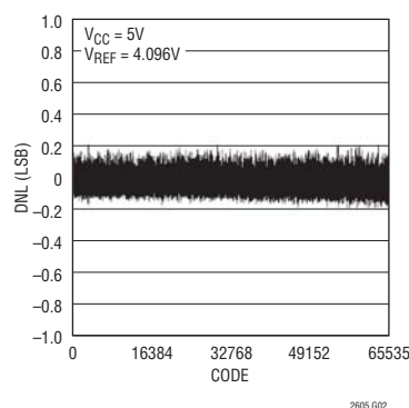
Differential Nonlinearity (LTC2605)
