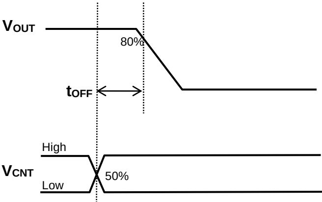
Fig.4 t_{OFF}
