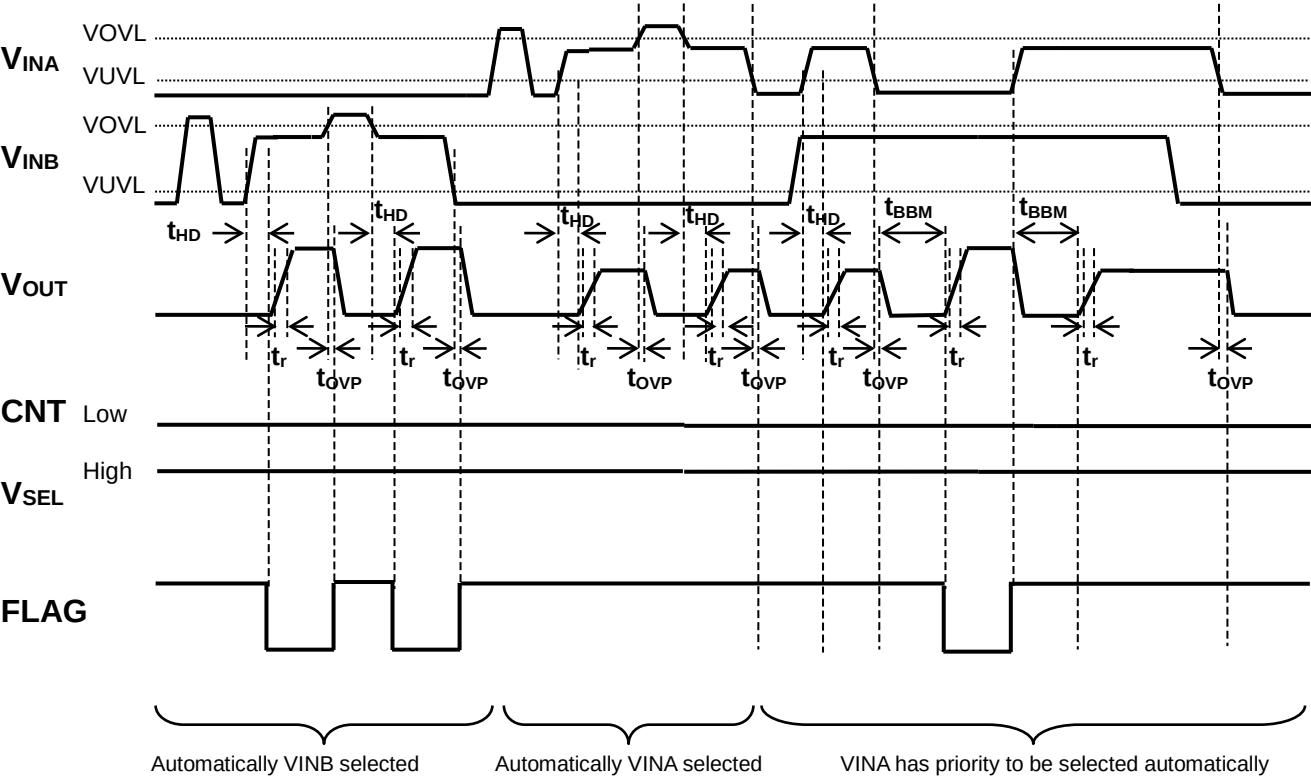
Fig.3 t_{HD} , t_{OVP}
