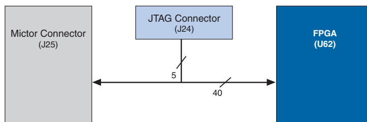
Figure 2–13. Mictor Connector Signaling
