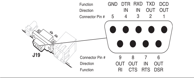
Figure 2-5. Serial Connector J19
