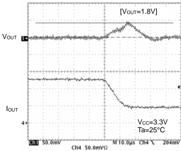
Figure 18. Transient Response ( I_o=125mA to 50mA , 10\mu s )
