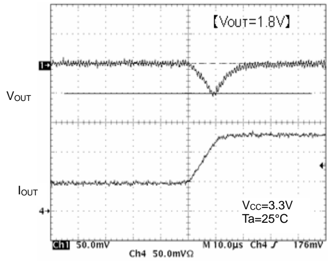
Figure 17. Transient Response ( I_o=50mA to 125mA , 10\mu s )
