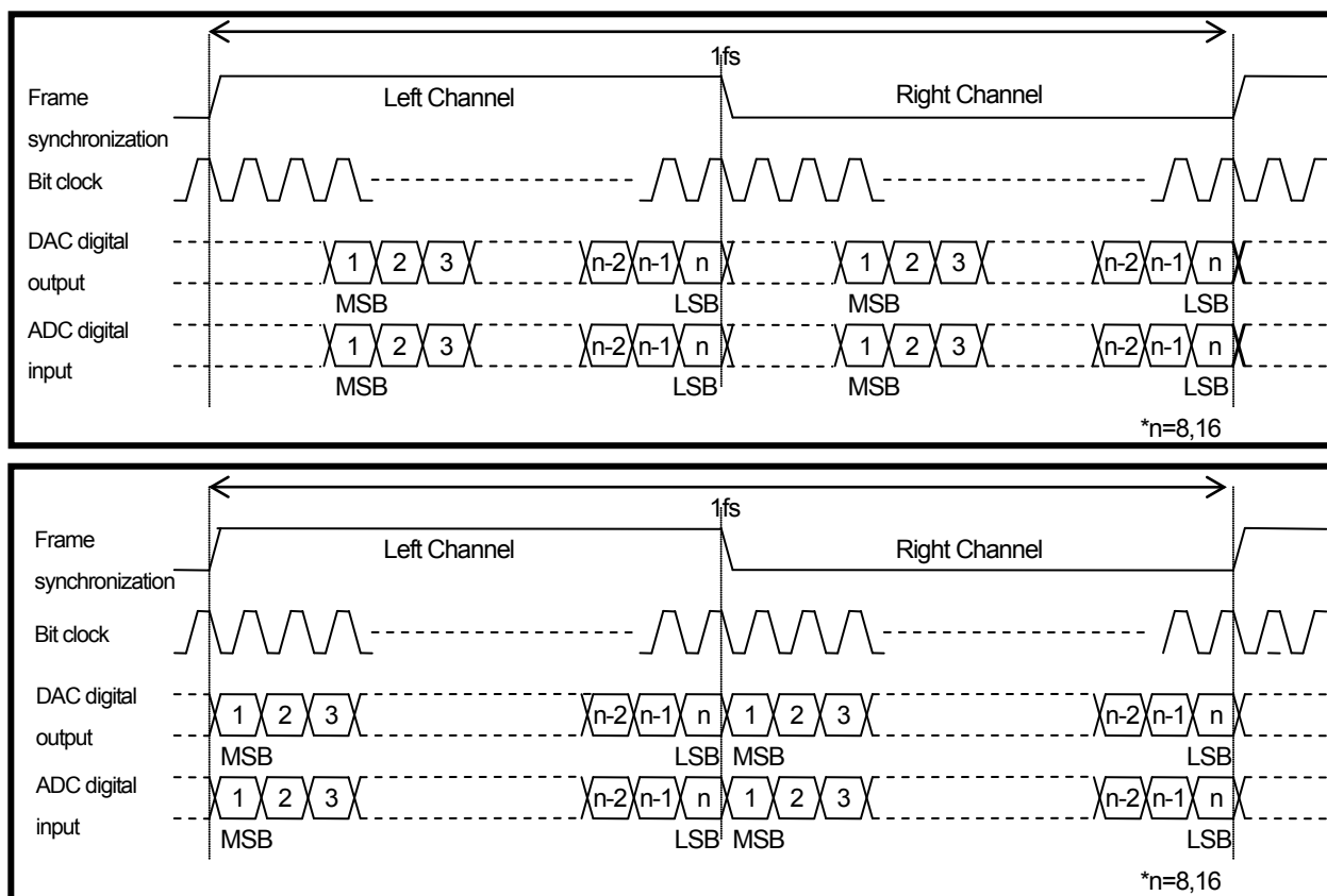
Figure 4-12 MSB right-justified format
