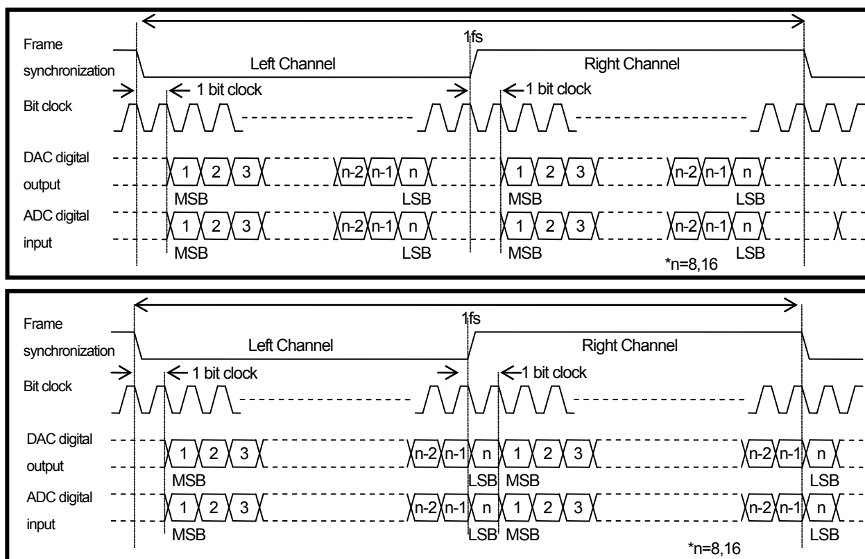
Figure 4-13 I 2 S format
