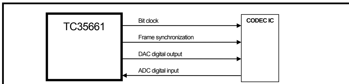
Figure 4-7 CODEC connection example (TC35661 is Master.)
