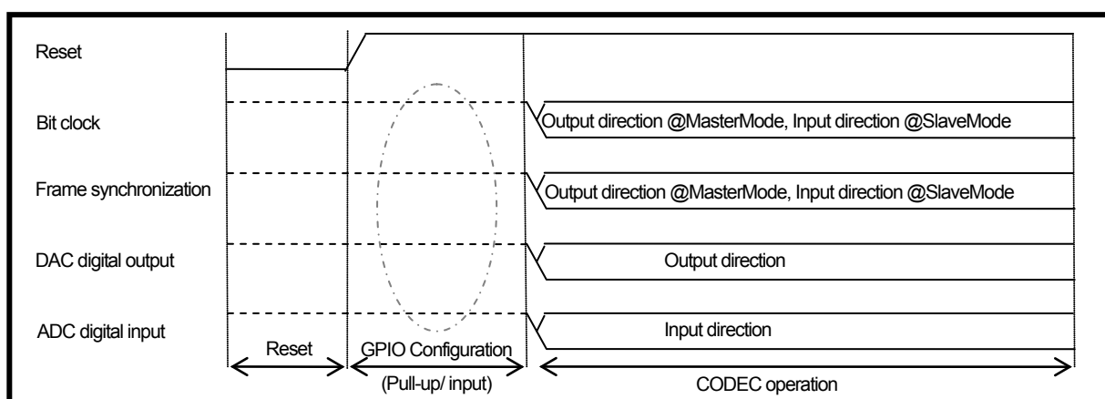
Figure 4-10 Assignment of CODEC interface function
