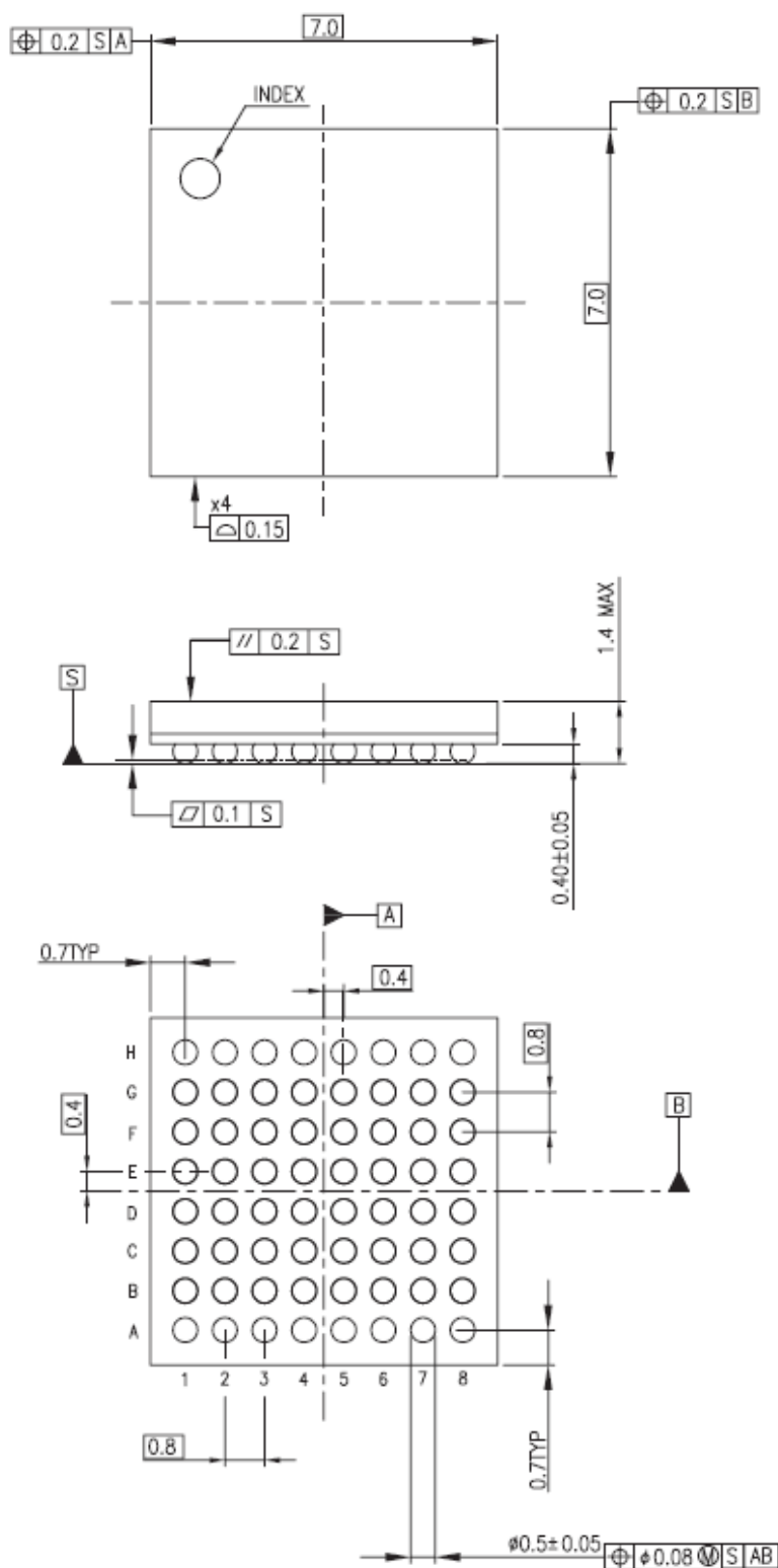
Figure 7-2 Package outline (P-LFBGA64-0707-0.80-001)
