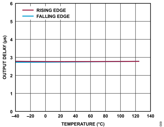
Figure 9. Output Delay vs. Temperature
