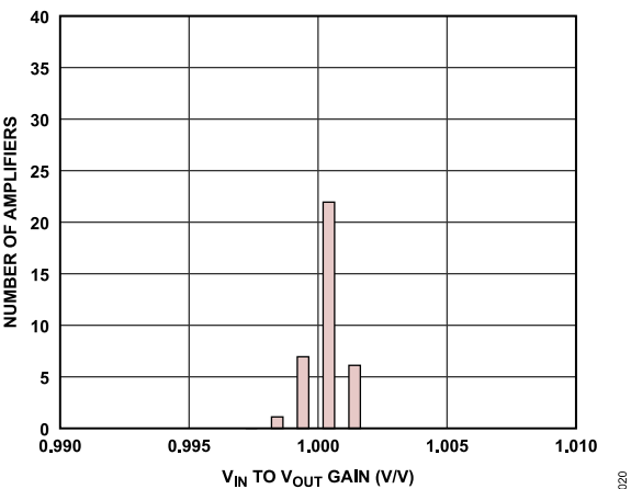
Figure 20. V_{IN} to V_{OUT} Gain Distribution at -40^{\circ}\text{C}
