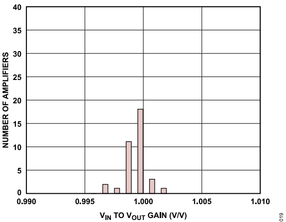
Figure 19. V_{IN} to V_{OUT} Gain Distribution at 125^{\circ}\text{C}
