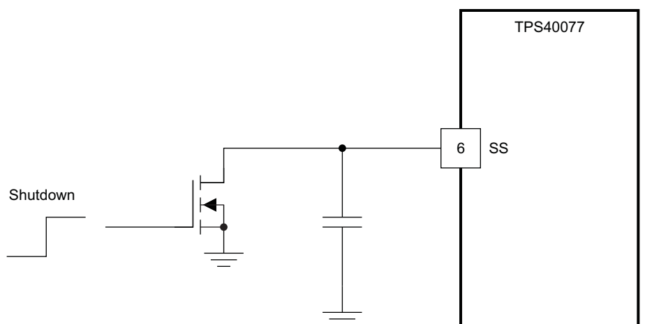
Figure 26. TPS40077 Shutdown
