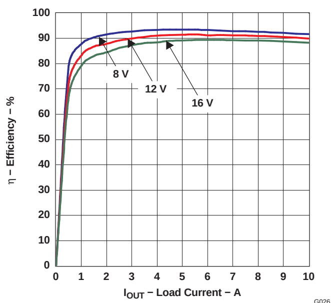
Figure 29. Module Efficiency, 8 V, 12 V, and 16 V In, 0 to 10 A Out
