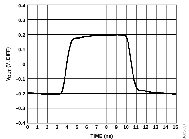
Figure 42. AD8117 Small Signal Pulse Response, 200 mV p-p
