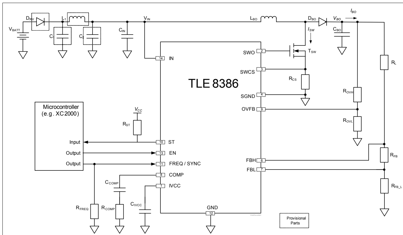
Figure 15 Boost Voltage Application Circuit (Current Source)
