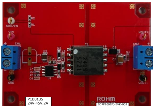
Figure 1. BD7F200EFJ-EVK-002 Evaluation Board
