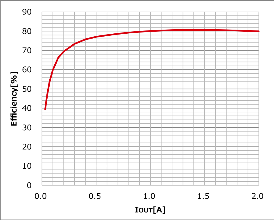
Figure 11. Efficiency vs Load Current
