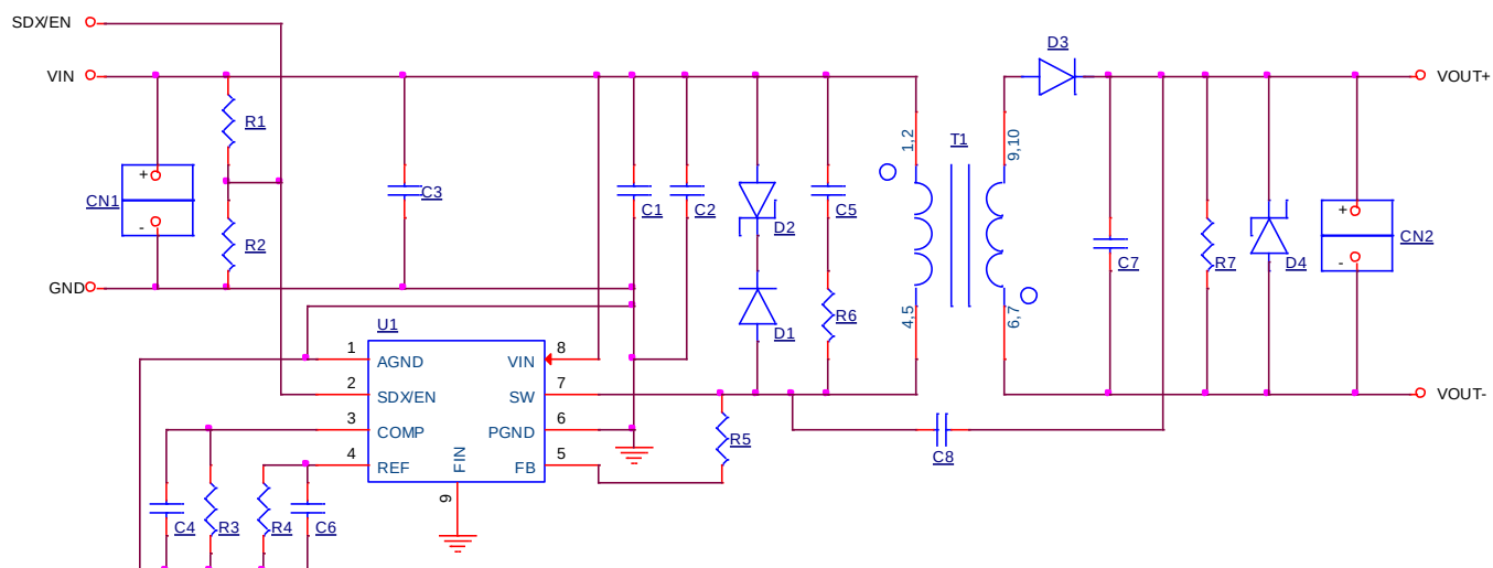
Figure 4. BD7F200EFJ-EVK-002 Circuit Diagram
