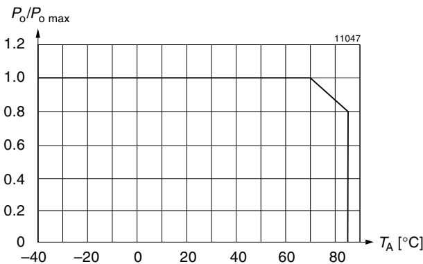
Fig. 21 Maximum allowed output power versus ambient temperature.
