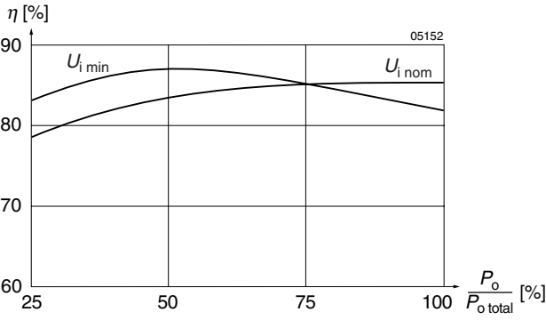
Fig. 11 Efficiency versus input voltage and load. Typical values IMY 35 D12D12-9
