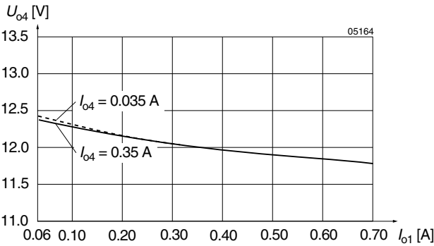
Fig. 9 Cross load regulation U_{o4} versus I_{o1} (typ) for various I_{o4} for Vo1, Vo4 on power train 1. See: Block diagram dual output types. (IMY 35 D12D12-9)
