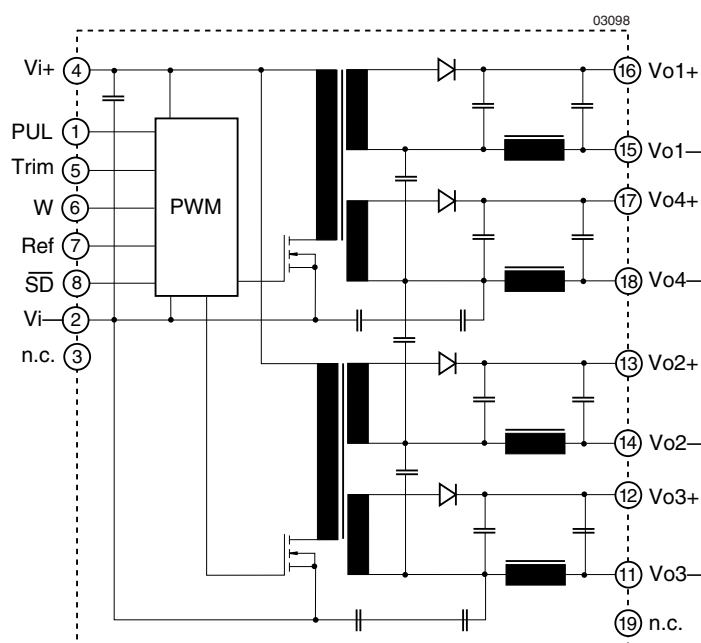
Fig. 2 Block diagram 3, quadruple output types
