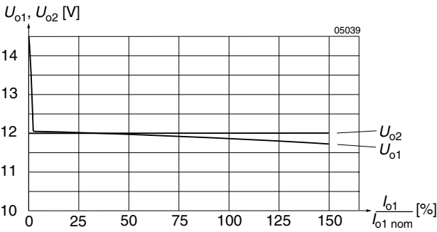
Fig. 10 Flexible load distribution on power train 1 of IMY 35 D12D12-9 ( 4 \times 12 V) with load variation from 0...150% of P_{o1 \text{ nom}} on output 1 (Vo1). Output 2 (Vo4) loaded with 50% of P_{o4 \text{ nom}} .
