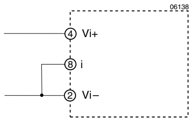
Fig. 22 If the inhibit is not used the inhibit pin should be connected to V_{i-}
