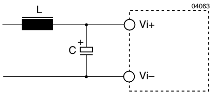
Fig. 5 Example for external circuitry to comply with IEC/EN 61000-4-5 or ETR 283 (19Pf11).
