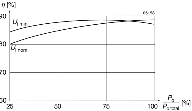
Fig. 12 Efficiency versus input voltage and load. Typical values IMY 35 D12D12-9
