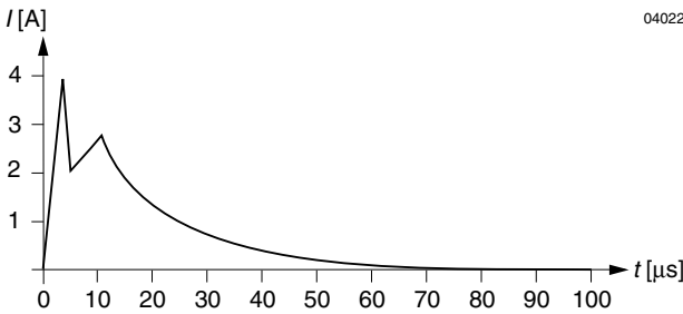
Fig. 3 Typical inrush current at U_{i\text{ nom}} , P_{o\text{ nom}} versus time. Source impedance according to prETS 300132-2, version 4.3 at U_{i\text{ nom}} .
