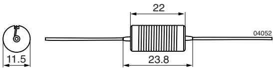
Fig. 6 Dimensions of inductor L for 110 IMY 35 types (e.g. Coil Craft, PCH-45 series).
