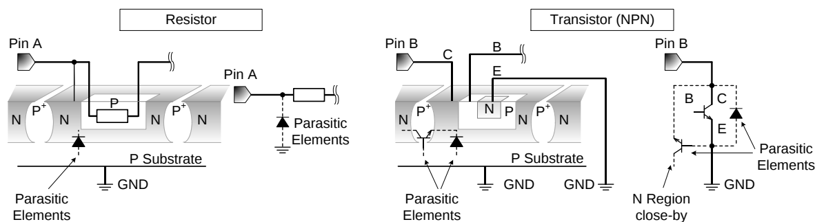
Figure 11. Example of IC Structure
