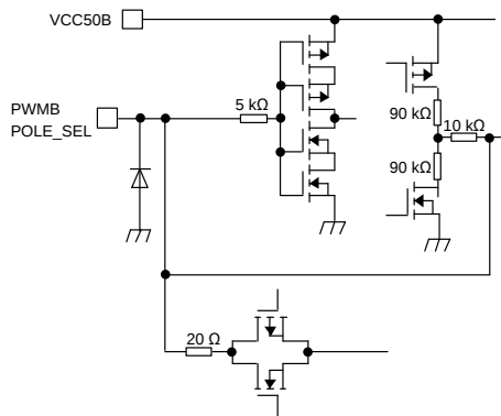
7) POLE_SEL, PWMB pin
