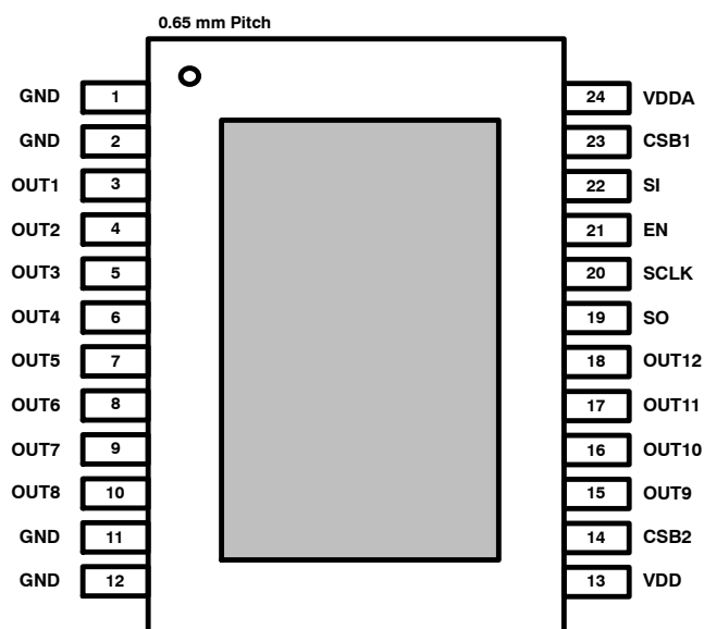
Figure 2. NCV7751 Pinout
