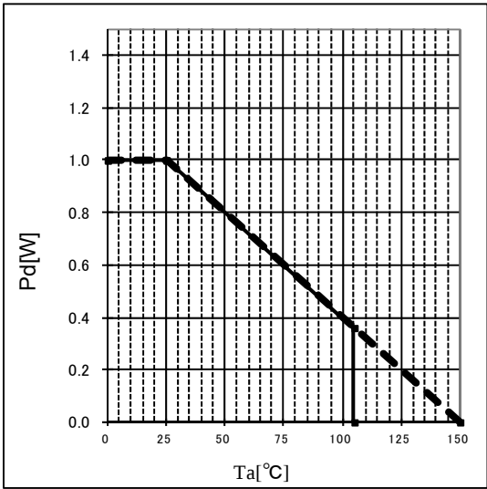
Figure 14. Thermal Abatement Characteristics
