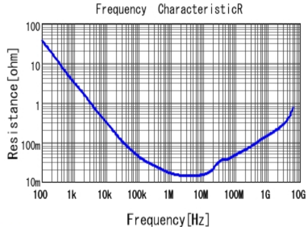
■ GRM155R61A334KE15 R DC0V, 25degC
