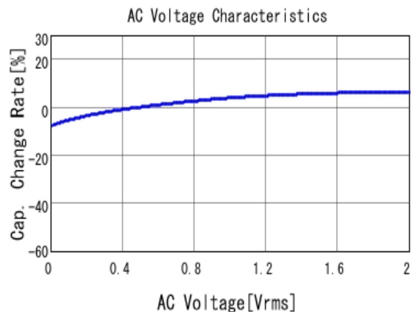
■ GRM155R61A334KE15 C-AC Voltage capchange, DC0V, 25.0d
