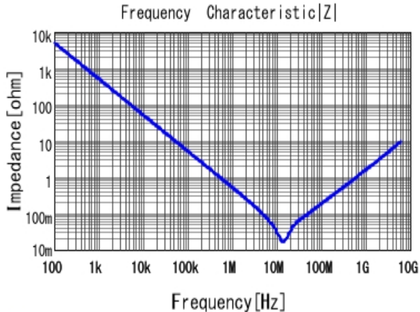
■ GRM155R61A334KE15 |Z| DC0V, 25degC
