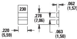
12 Screwdriver Slot (with marking)
