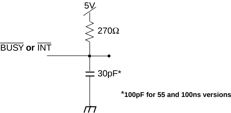
Figure 3. \overline{\text{BUSY}} and \overline{\text{INT}} AC Output Test Load
