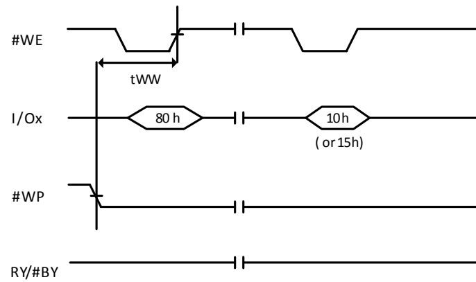
Figure 9-26 Program Disable
