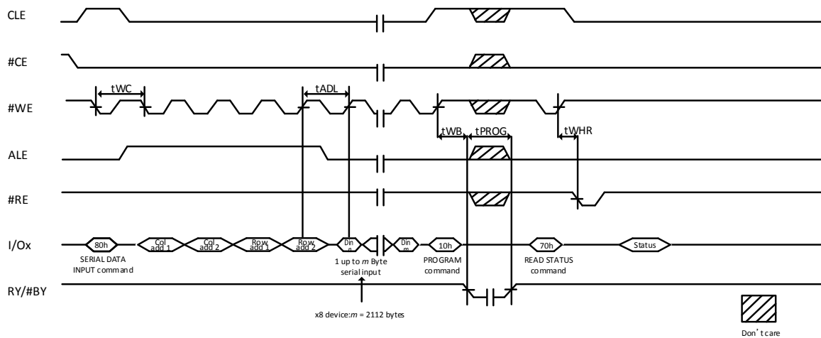
Figure 11-11 Page Program
