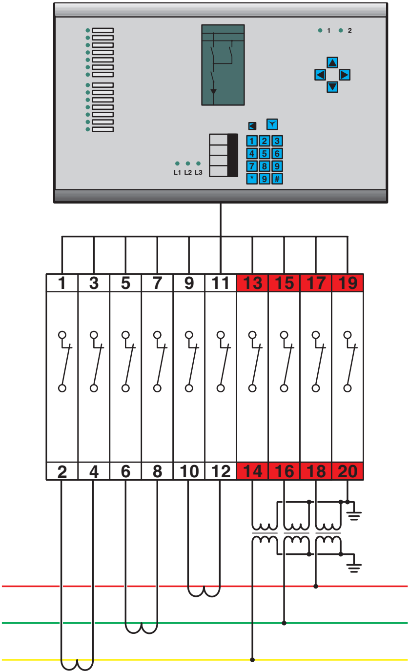
Circuit diagram
