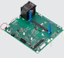
Half-Bridge Motherboard
