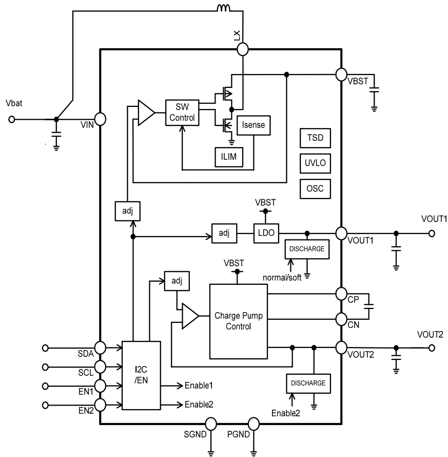
Fig.2 Block Diagram
