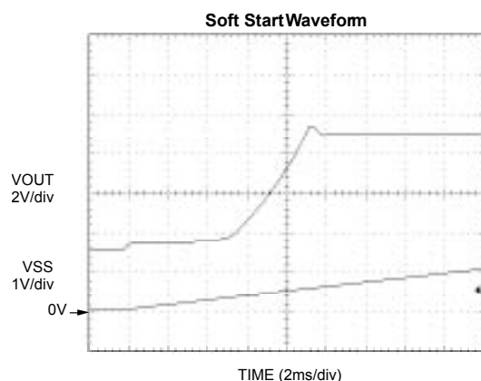
Figure 10 Soft Start
