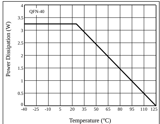
Figure 17 Dissipation Curve
