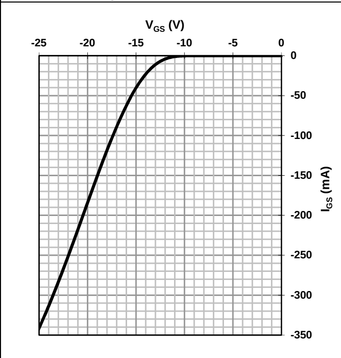
Figure 12 Typ. gate characteristics reverse
