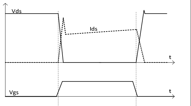
Figure 26 Typical Reverse Channel Recovery
