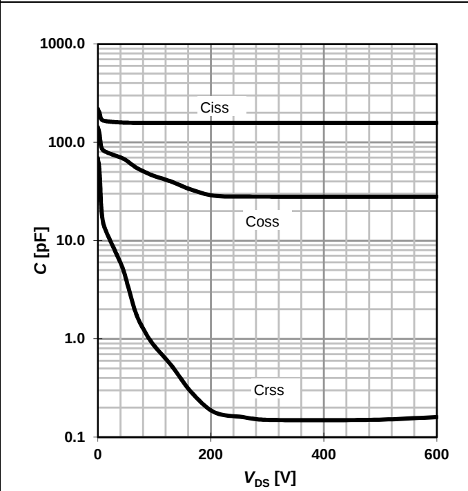
Figure 20 Typ. capacitances
