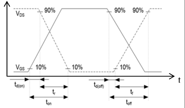
Figure 24 Switching times waveform
