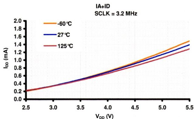
Figure 2. I_{DD} vs V_{DD} ( f_{SCLK}=3.2MHz )
