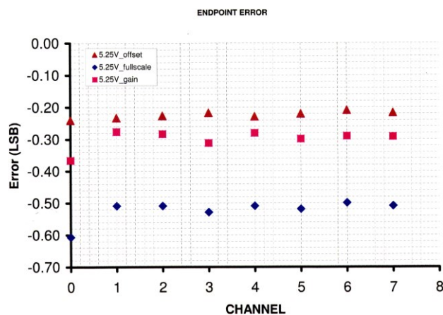
Figure 4. ENDPOINT ERROR vs CHANNEL ( V_{DD}=5.25V )
