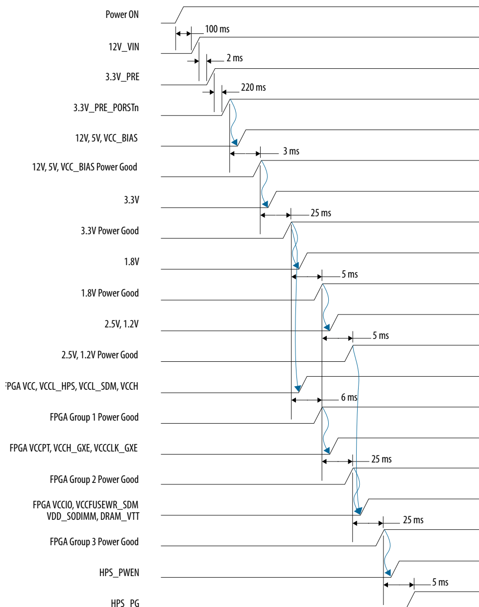
Figure 18. Power Sequence
