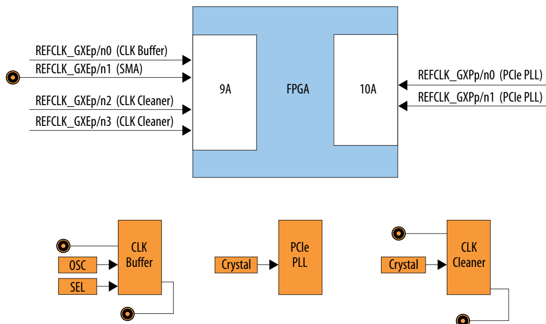
Figure 20. Transceiver Clocks
