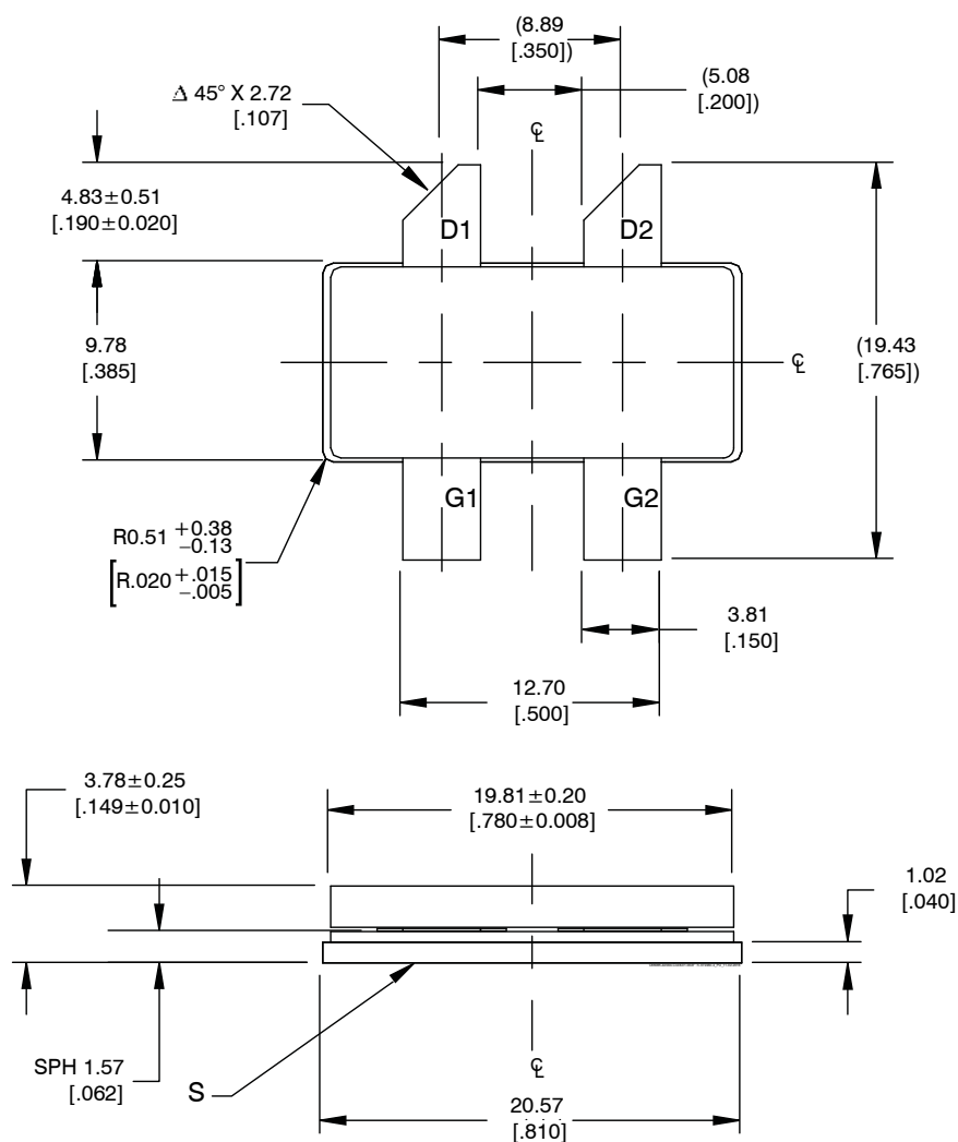
Package H-37248C-4
