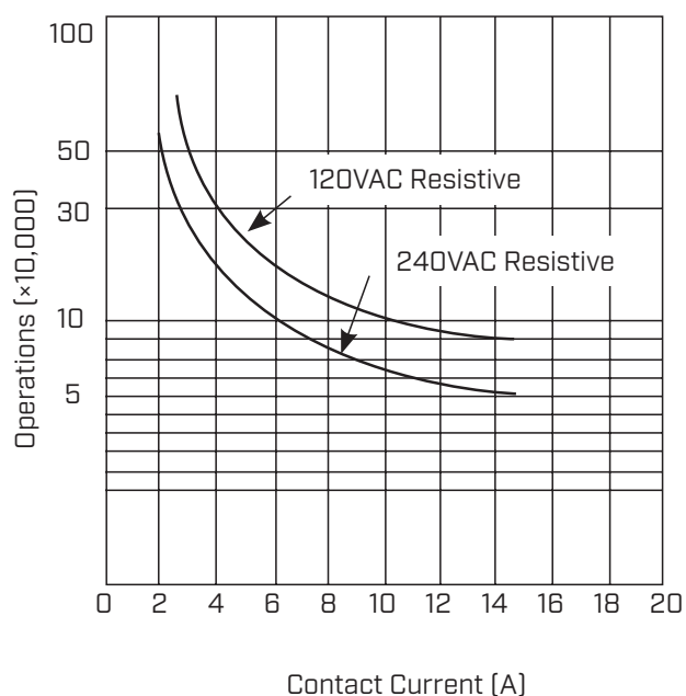
Life Curve
