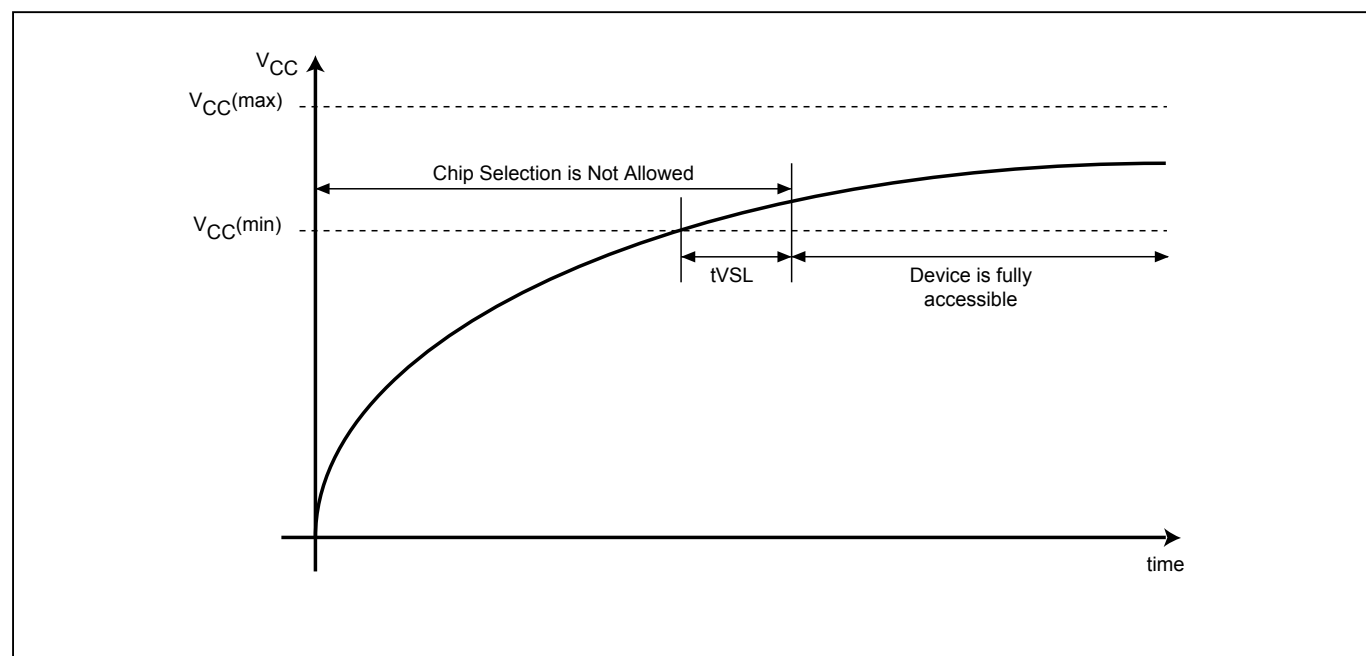
Figure 34. Power-up Timing
