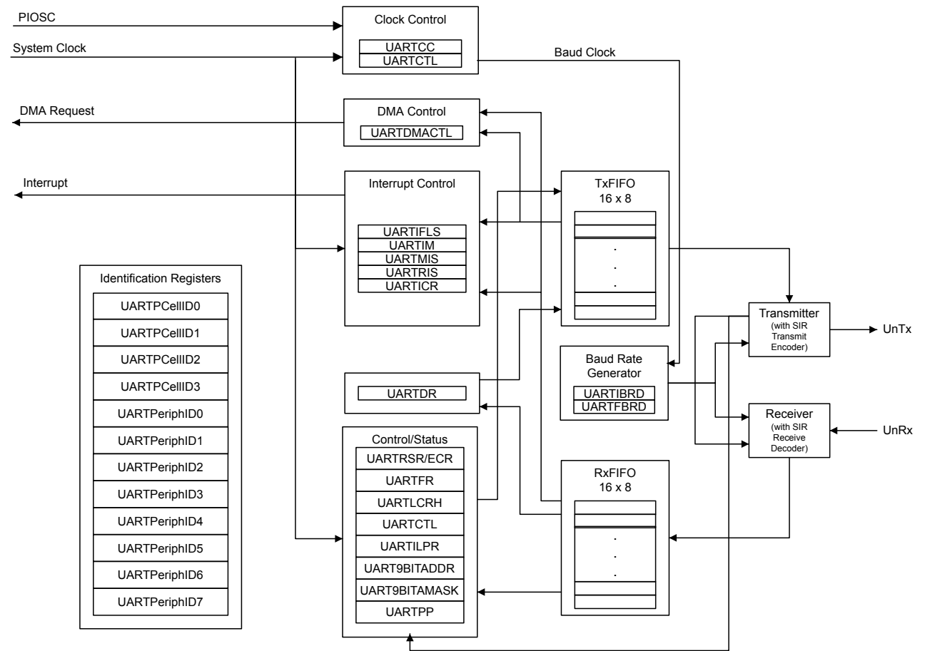
Figure 14-1. UART Module Block Diagram
