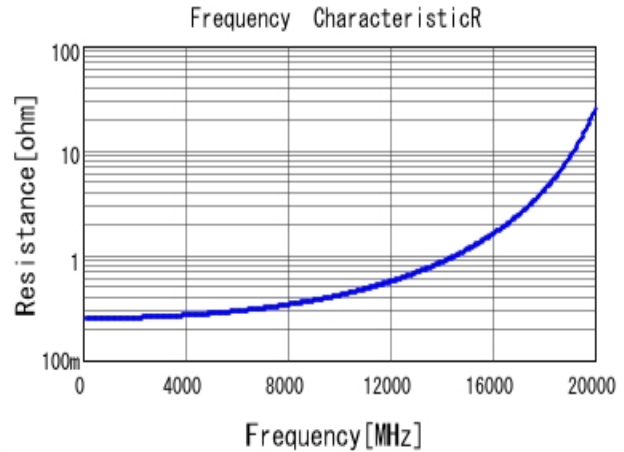
■ GCQ1555C1HR90BB01 R DC0V, 25degC
