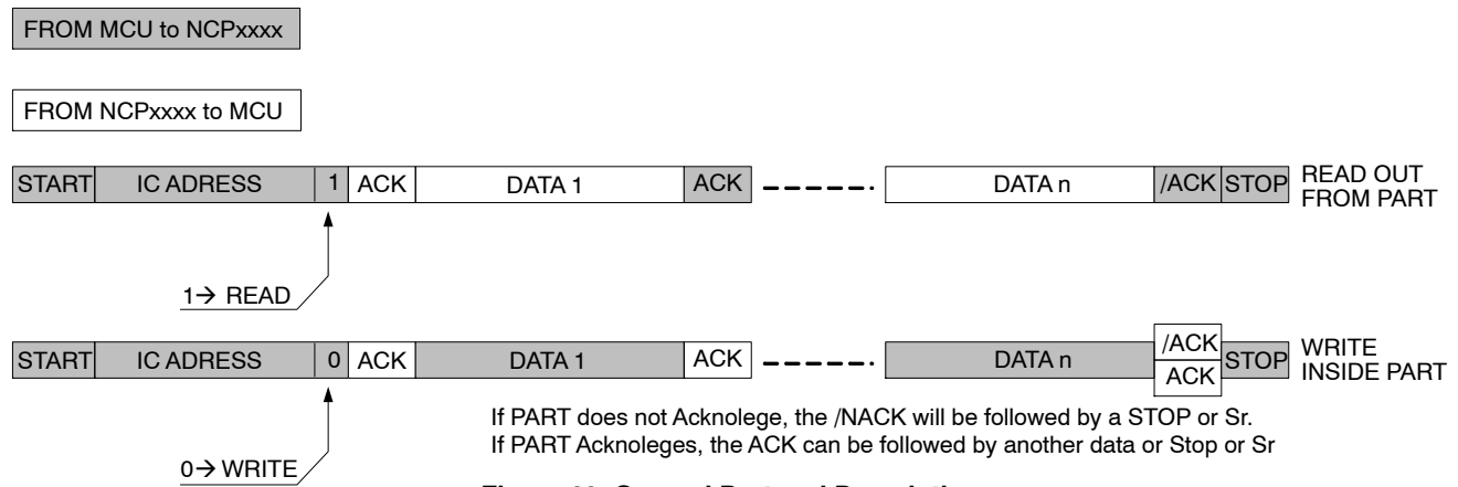
Figure 69. General Protocol Description
