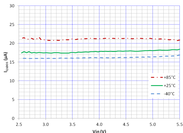
Figure 29. I_{\text{Q LDO3}} vs V_{\text{IN}} and Temperature
