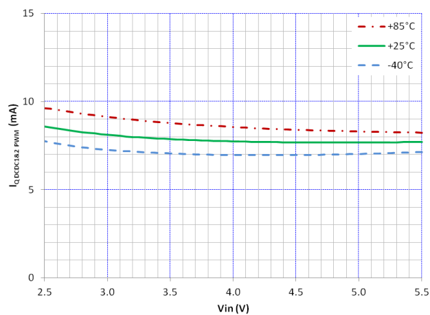
Figure 31. I_{\text{Q PWM}} vs V_{\text{IN}} and Temperature
