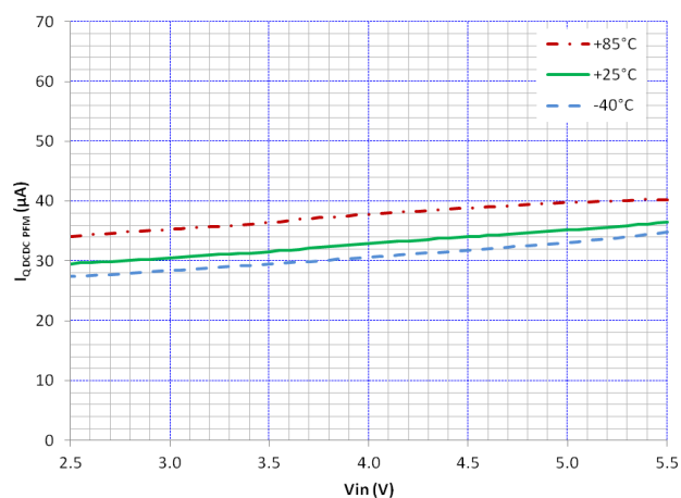
Figure 30. I_{\text{Q PFM}} vs V_{\text{IN}} and Temperature
