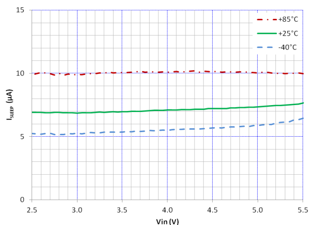
Figure 28. I_{\text{SLEEP}} vs V_{\text{IN}} and Temperature
