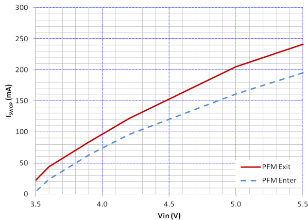
Figure 27. DCDC2 Switchover Point V_{OUT} = 3.30\text{V}
