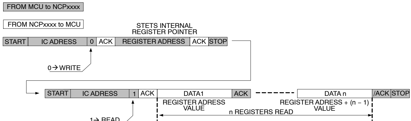
Figure 70. Read Out from Part
