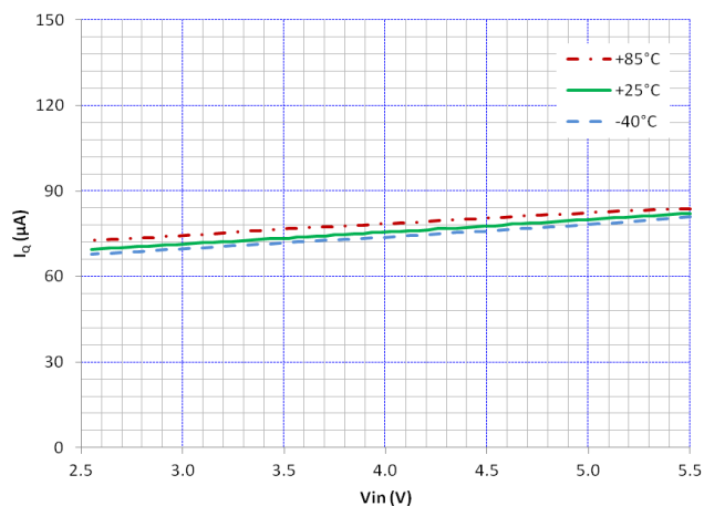
Figure 32. I_{\text{Q}} vs V_{\text{IN}} and Temperature
