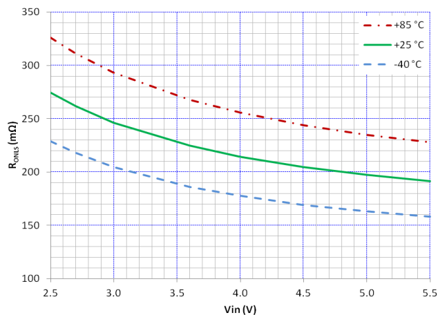
Figure 25. DCDC2 LSS R_{ON} vs V_{IN} and Temperature
