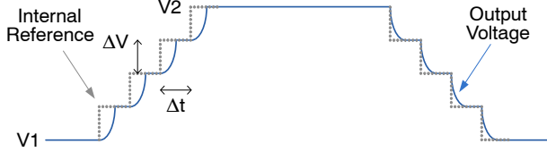
Figure 60. Default Dynamic Voltage Scaling Effect Timing Diagram
