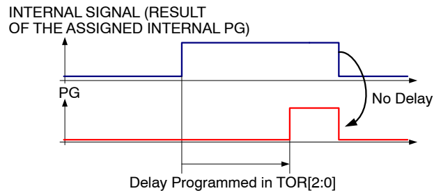
Figure 66. PG Delay
