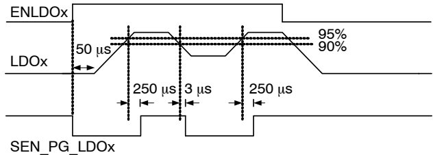
Figure 62. DCDCx Channel Internal Power Good Signal
