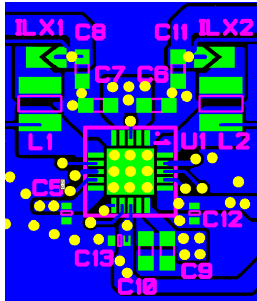
Figure 74. Recommended PCB Layout
