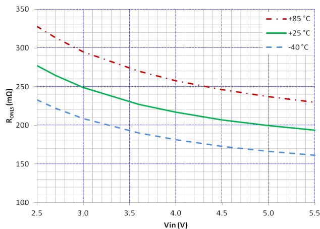
Figure 23. DCDC1 LSS R_{ON} vs V_{IN} and Temperature
