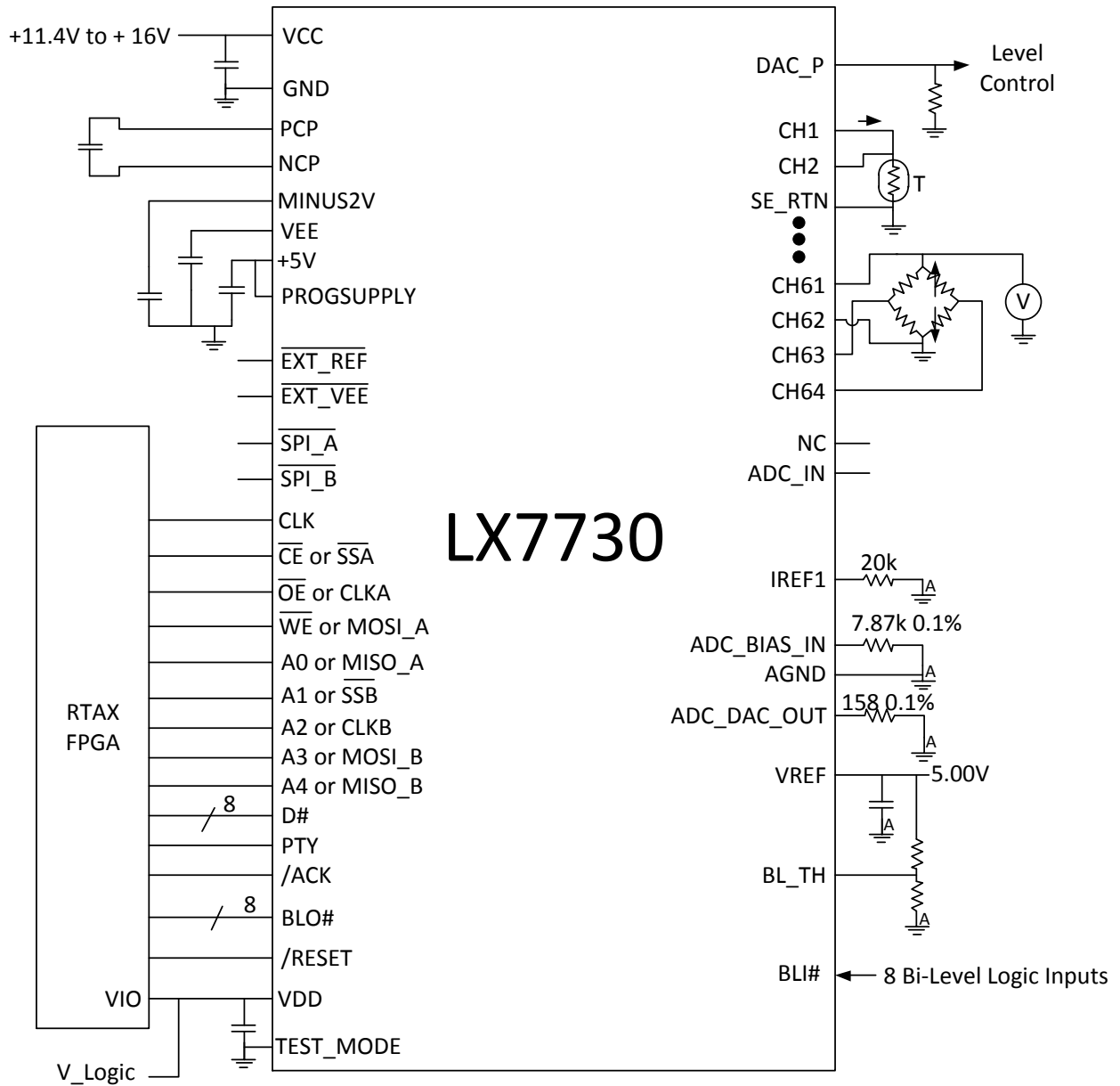
Figure 5 · Typical Application
