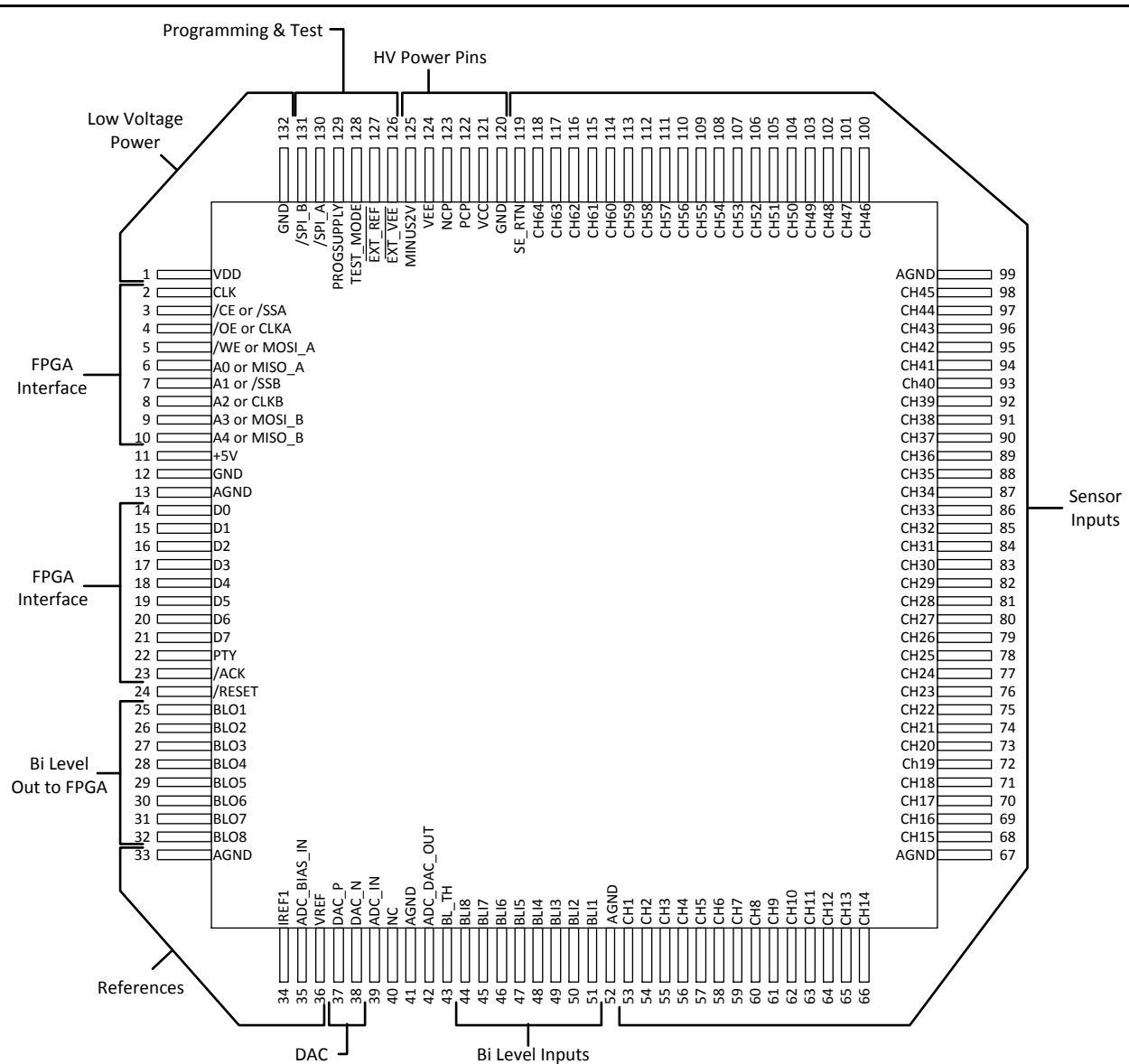
Figure 2 · Pinout
