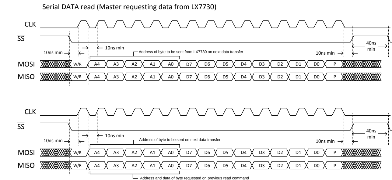
Figure 7 · Serial Data Read Timing Diagram
