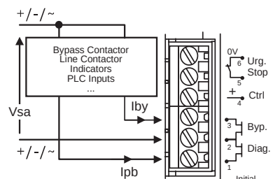
Fig. 6 STATUS OUTPUT UTILIZATION
