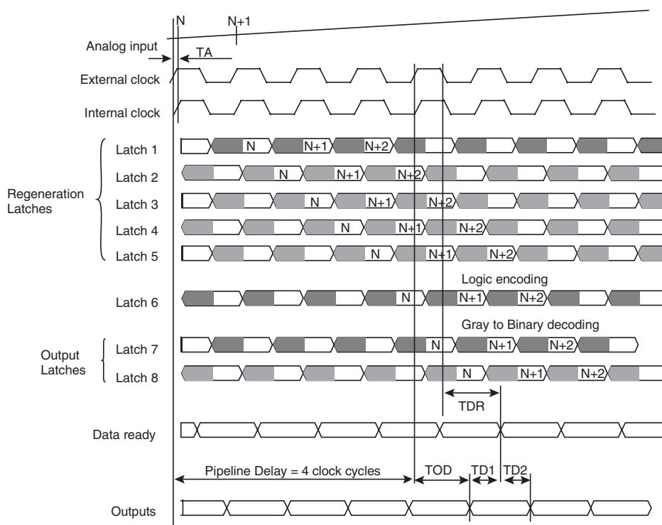
Figure 3-1. Timing Diagram
