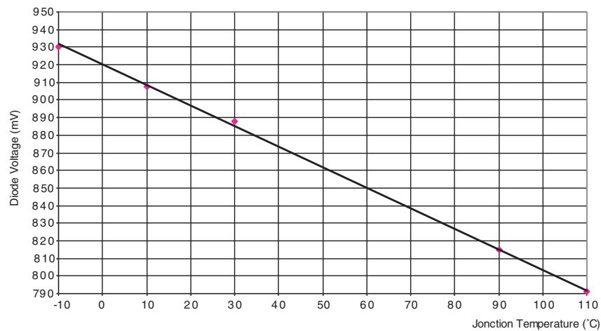
Figure 9-15. Junction Temperature vs. Diode Voltage for I = 1 \text{ mA}
