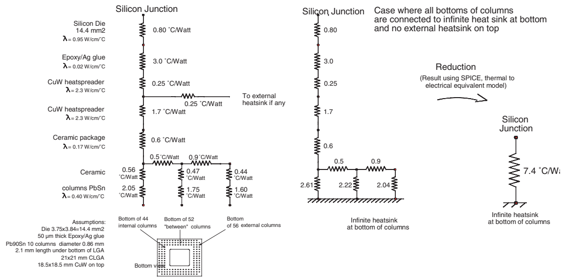
Figure 5-2. Thermal Net
