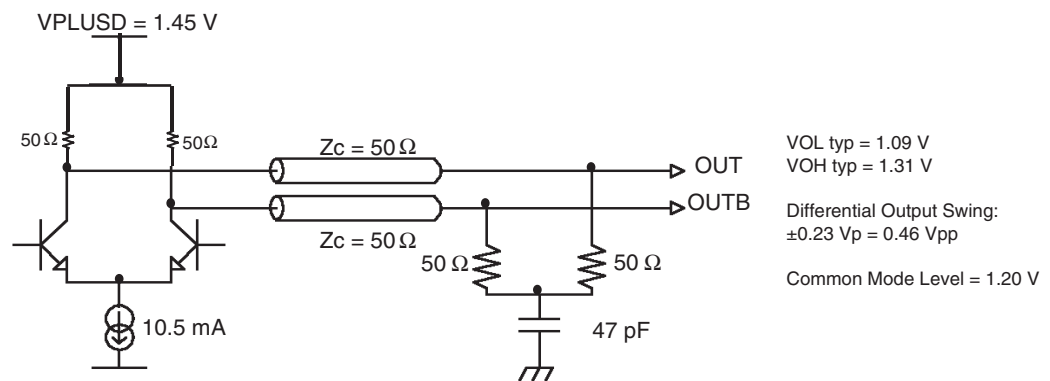
Figure 9-9. 50 Ω Terminated Differential Outputs (Recommended)
