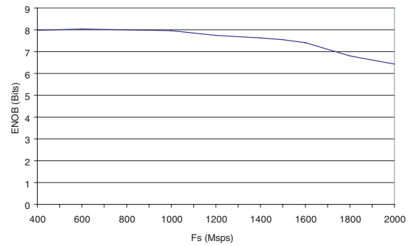
Figure 6-5. ENOB vs. Sampling Frequency in Nyquist Conditions ( F_{in} = F_s/2 )
