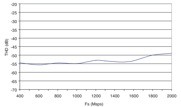
Figure 6-7. THD vs. Sampling Frequency in Nyquist Conditions ( F_{in} = F_s/2 )
