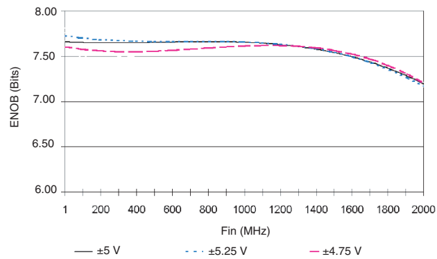
Figure 6-23. ENOB vs. V_{CC} and V_{EE} ; F_s = 1.4 Gsps vs. F_{in} ( V_{CC} = |V_{EE}| = 4.75V, 5V and 5.25V )
