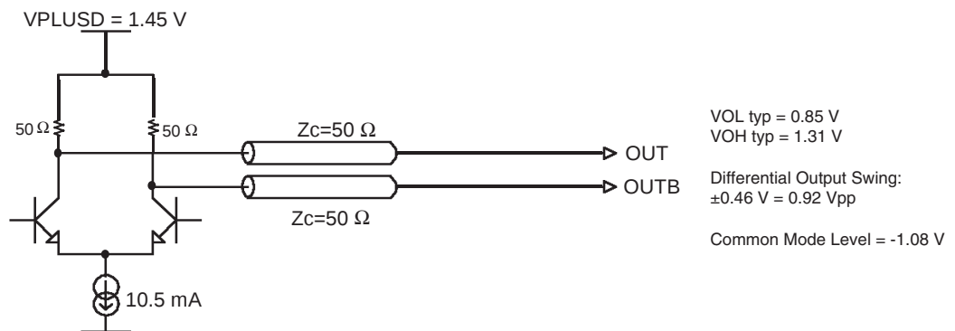
Figure 9-10. Unterminated Differential Outputs (Optional)
