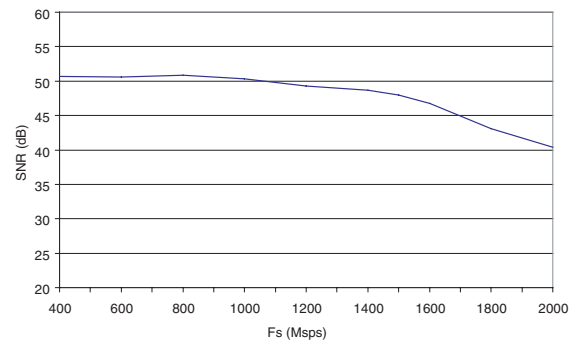
Figure 6-8. SNR vs. Sampling Frequency in Nyquist Conditions ( F_{in} = F_s/2 )
