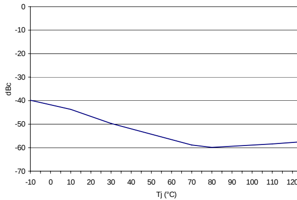
Figure 6-21. SFDR vs. Junction Temperature ( F_s = 1.4 Gsps, F_{in} = 698 MHz, -1 dBFS)
