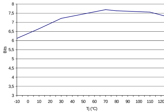
Figure 6-20. ENOB vs. Junction Temperature ( F_s = 1.4 Gsps, F_{in} = 698 MHz, -1 dBFS)
