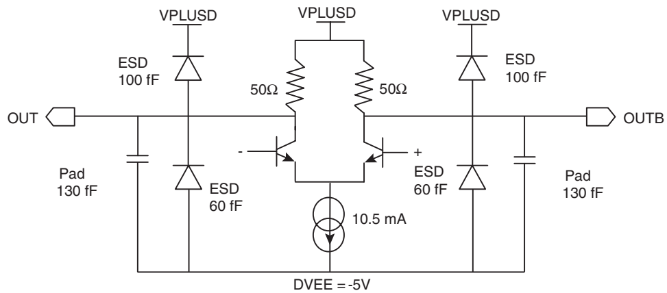
Figure 7-3. Equivalent Data Output Buffer Circuit and ESD Protections
