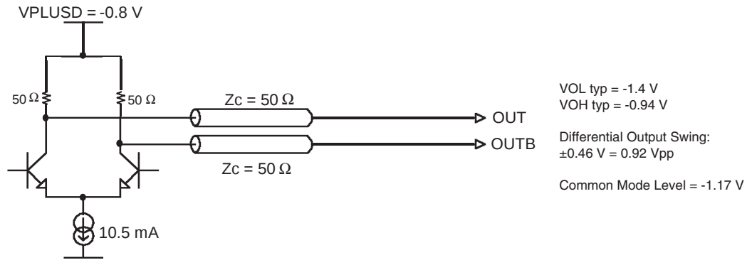
Figure 9-8. Unterminated Differential Outputs (Optional)
