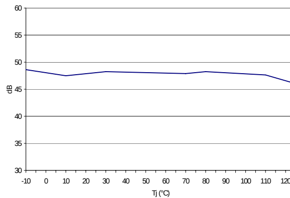
Figure 6-22. SNR vs. Junction Temperature ( F_s = 1.4 Gsps, F_{in} = 698 MHz, -1 dBFS)
