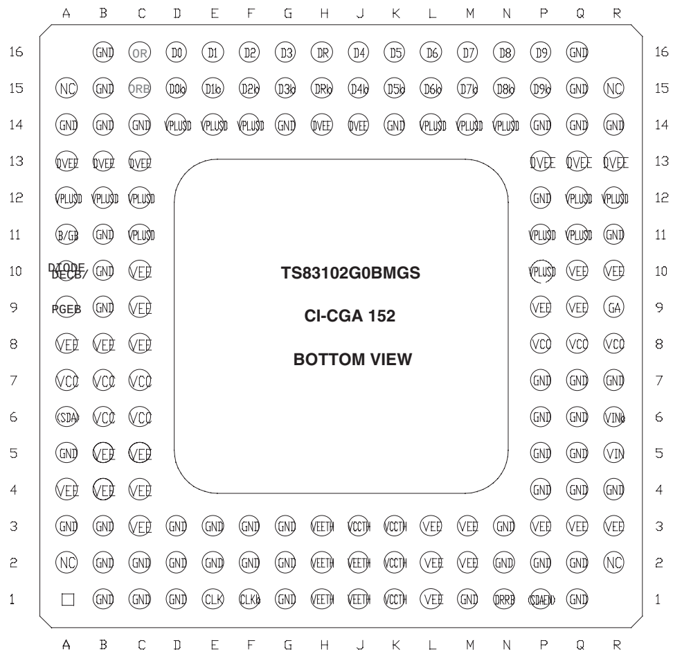
Figure 4-1. Pinout
