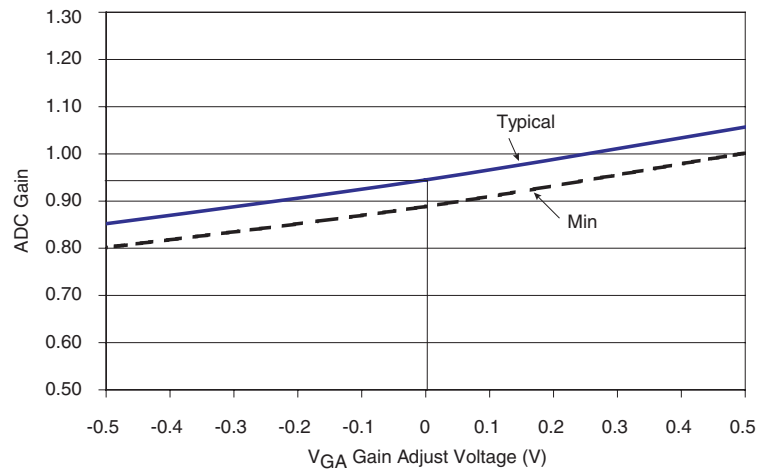
Figure 9-16. Gain Adjust Transfer Function
