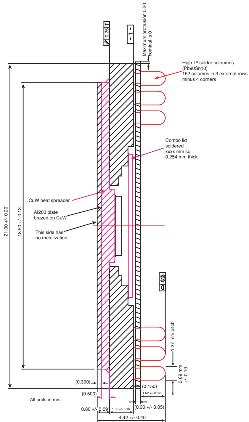
Figure 11-3. Cross Section
