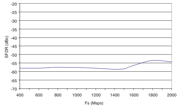
Figure 6-6. SFDR vs. Sampling Frequency in Nyquist Conditions ( F_{in} = F_s/2 )
