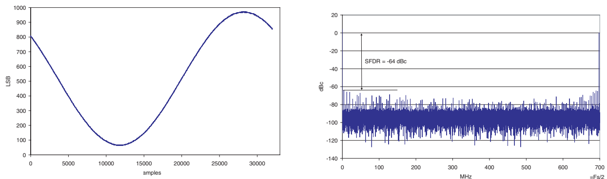
Figure 6-13. F_s = 1.4 Gsps and F_{in} = 702 MHz, -1 dBFS; Decimation Factor = 8, 32 kpoints FFT
