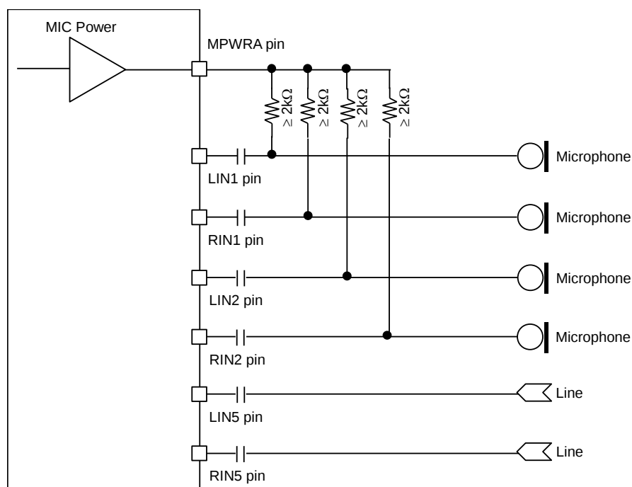
Figure 41. ADCA MIC Block Circuit MDIFA (MDIFA1=MDIFA2="0")
