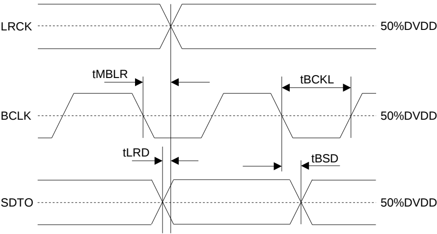
Figure 3. Audio Interface Timing (PLL/EXT Master mode & Normal mode)
