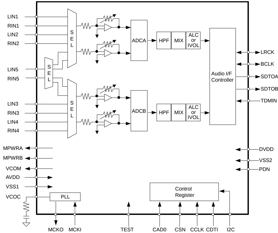
Figure 1. Block Diagram
