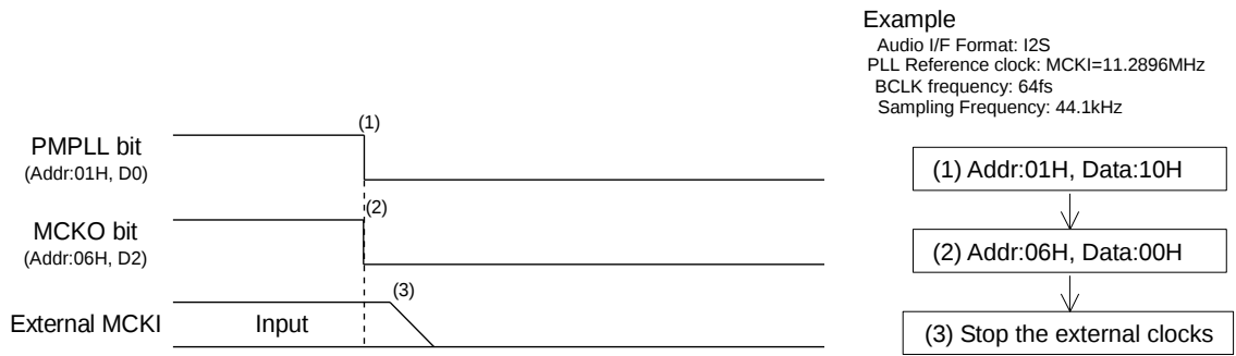
Figure 67. Clock Stopping Sequence (3)
