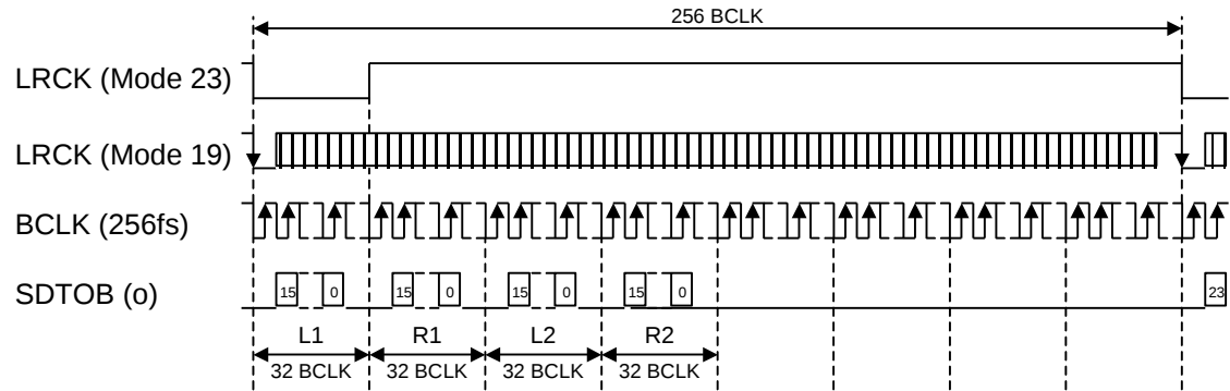
Figure 34. Mode 19, 23 Timing (TDM256 mode, I 2 S compatible)
