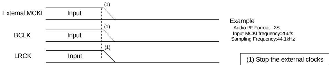
Figure 68. Clock Stopping Sequence (4)
