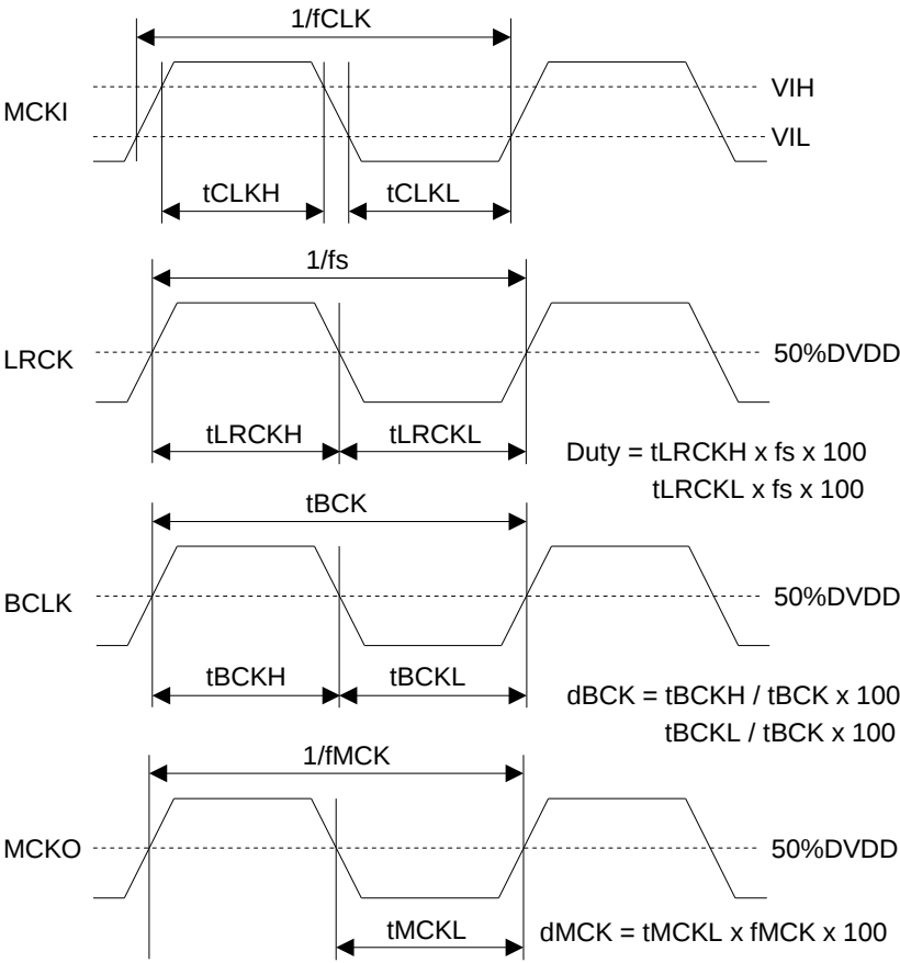
Figure 2. Clock Timing (PLL/EXT Master mode)
