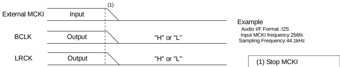
Figure 69. Clock Stopping Sequence (5)
