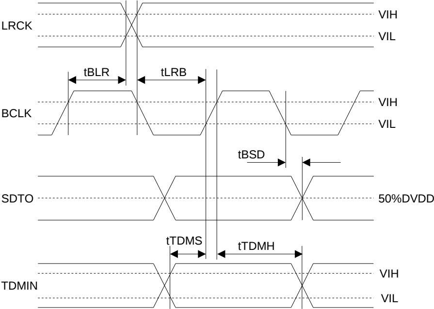
Figure 13. Audio Interface Timing (PLL/EXT Slave mode)
