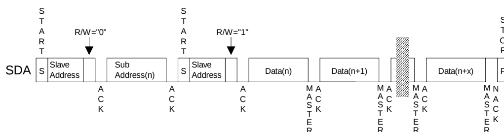
Figure 52. RANDOM ADDRESS READ
