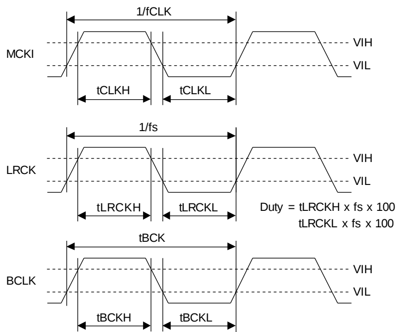
Figure 12. Clock Timing (EXT Slave mode)
