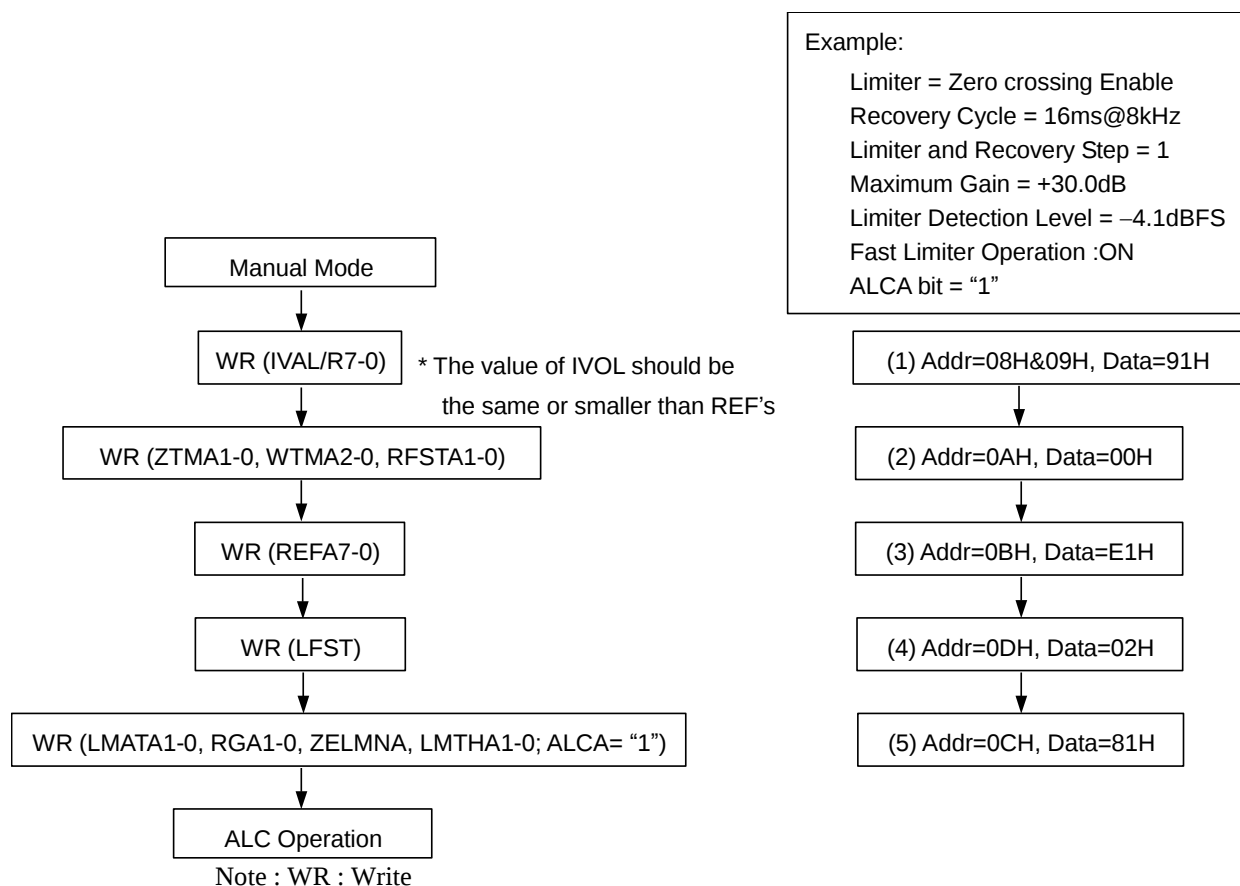
Figure 43. Registers set-up sequence at ALCA operation
