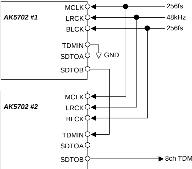
Figure 37. Cascade TDM Connection example (TDM256, MSB justified)
