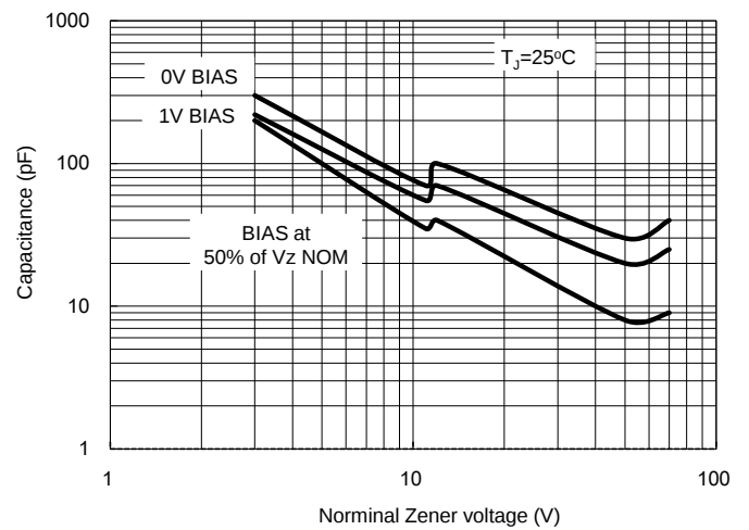
Fig. 4 Typical capacitance
