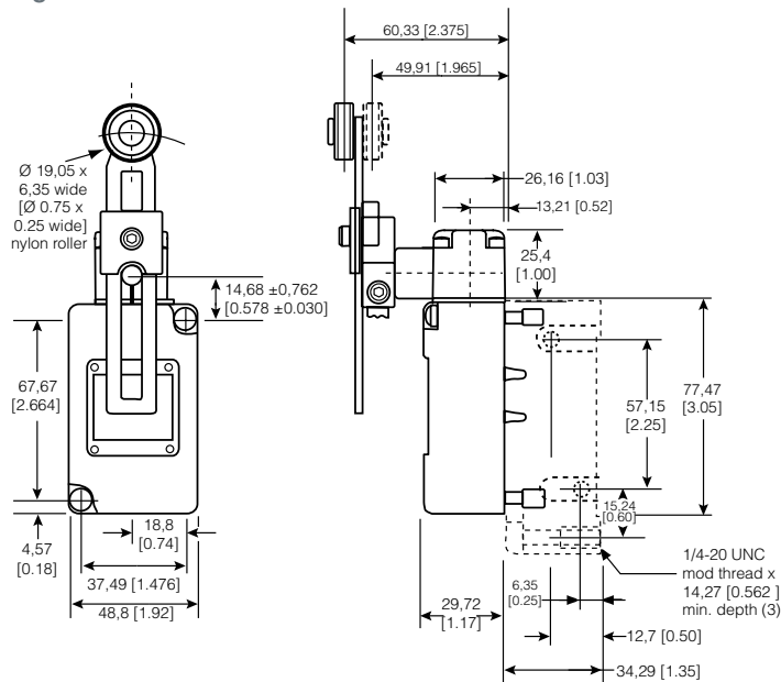
Figure 13. 201LS3 Dimensions
