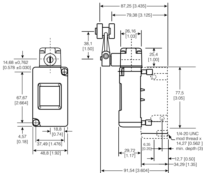
Figure 13. 201LS3 Dimensions
