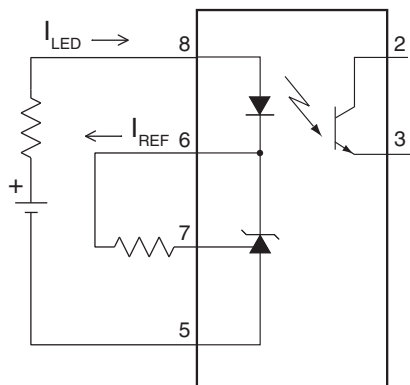
I_{REF} Test Circuit
