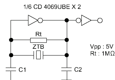
Figure 3) Test Circuit
