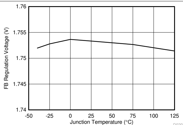
Figure 6-13. Feedback Regulation Voltage vs Temperature
