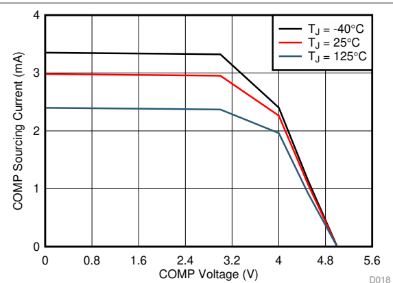
Figure 6-18. Error Amplifier Source Current
