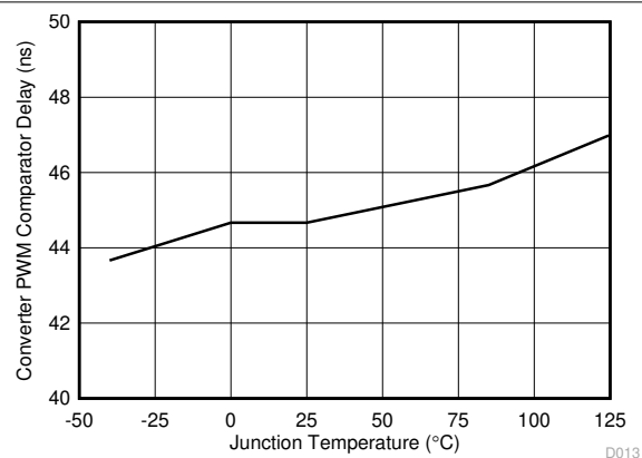
Figure 6-16. Converter PWM Comparator Delay vs Temperature
