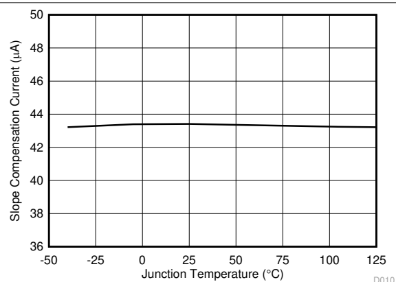
Figure 6-14. Current Slope Compensation Current vs Temperature
