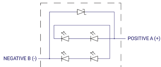
12-V Configuration
