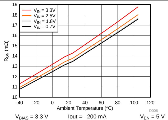
Figure 8. R_{ON} vs Temperature, V_{BIAS} = 3.3 V
