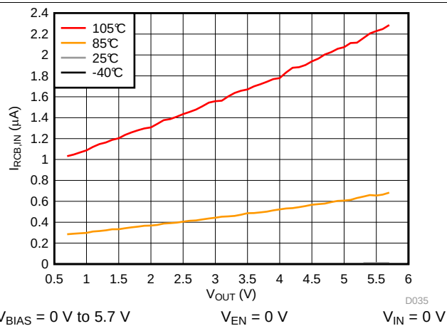
Figure 5. I_{RCB,IN} vs V_{OUT}
