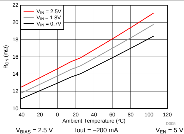
Figure 7. R_{ON} vs Temperature, V_{BIAS} = 2.5 V
