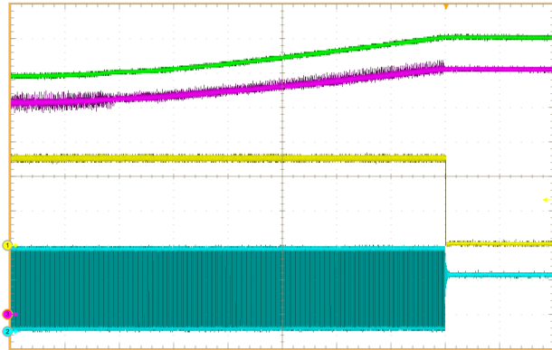
Figure 29. OVP1 at V_{FB} \geq 115\% V_{REF}
