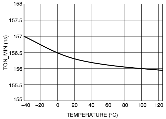
Figure 17. T_{ON\_MIN} vs. T at V_{HVBias} = 48\text{ V}
