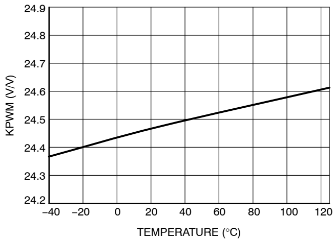
Figure 16. PWM Modulator Gain, V_{IN} / \Delta V_{RAMP} vs. T at V_{HVBias} = 48\text{ V}
