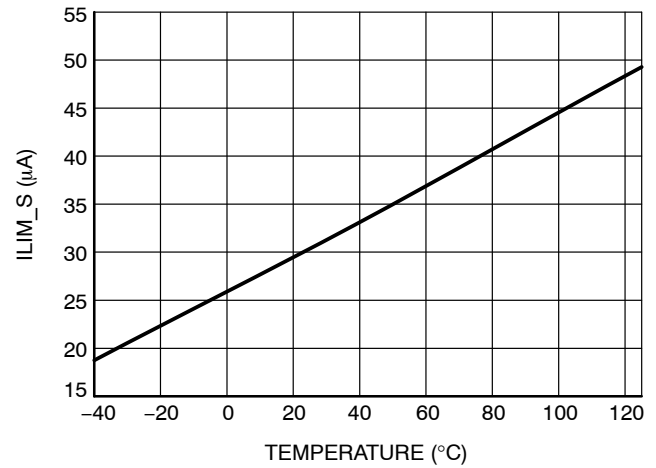
Figure 19. 30\text{ }\mu\text{A} Current Source for Current Limit Purpose vs. T at V_{HVBias} = 48\text{ V}
