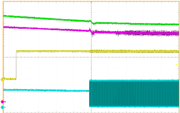
Figure 30. OVP1 Release at V_{FB} \leq 110\% V_{REF}
