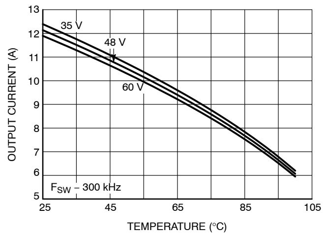
Figure 38. Thermal De-rating Curve
