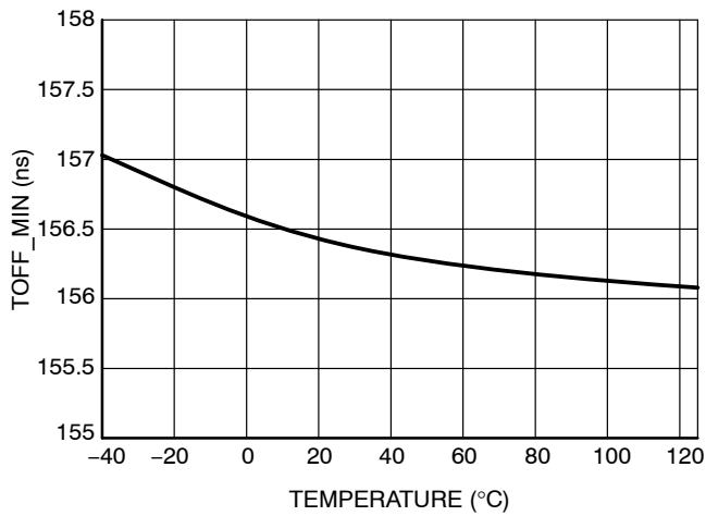
Figure 18. T_{OFF\_MIN} vs. T at V_{HVBias} = 48\text{ V}
