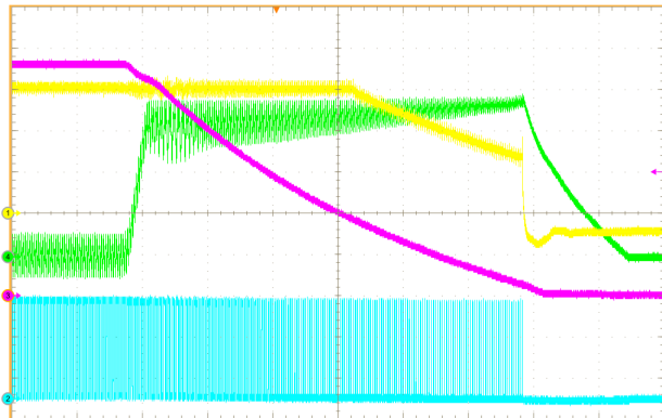
Figure 31. UVP due to Deep Over-current
