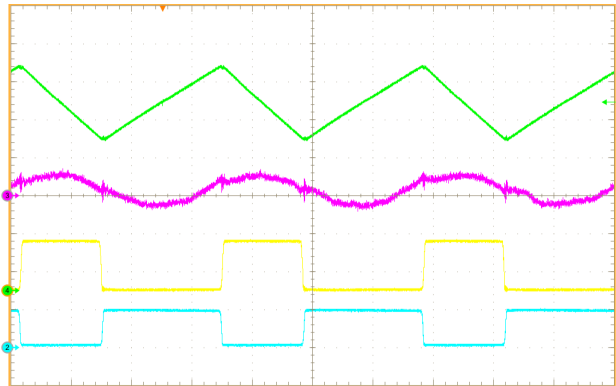
Figure 32. Switching and Voltage Ripple
