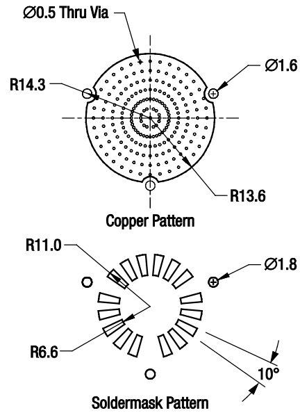
Recommended Footprint
