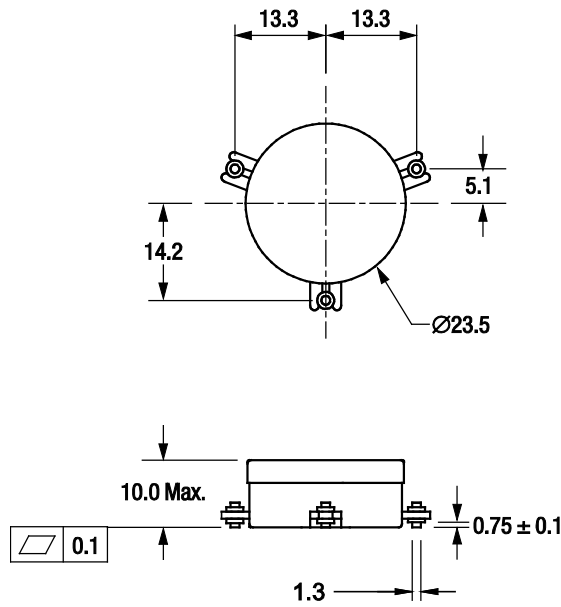
Package Dimensions
