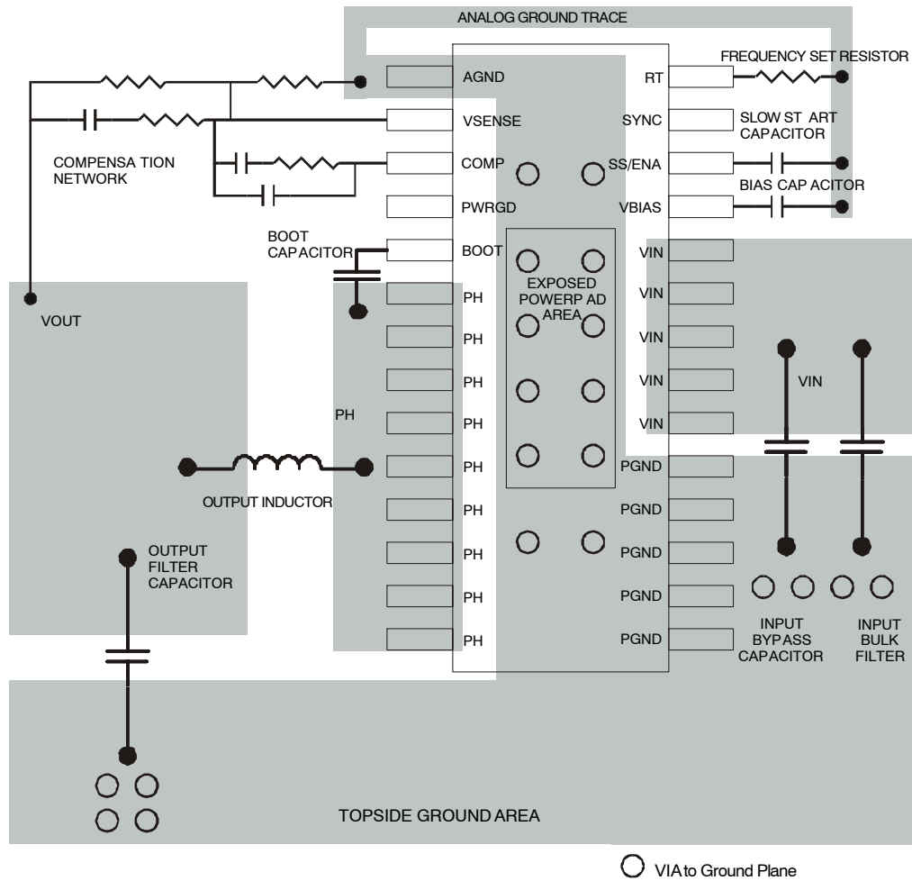
Figure 10. PCB Layout
