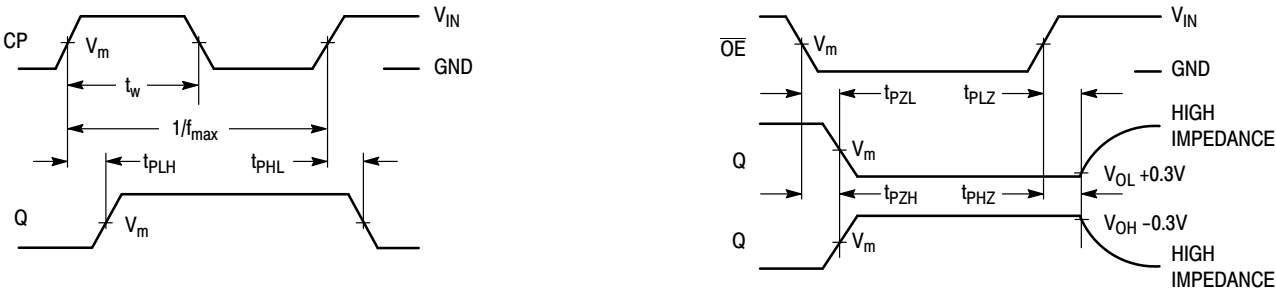
Figure 3. Switching Waveforms
