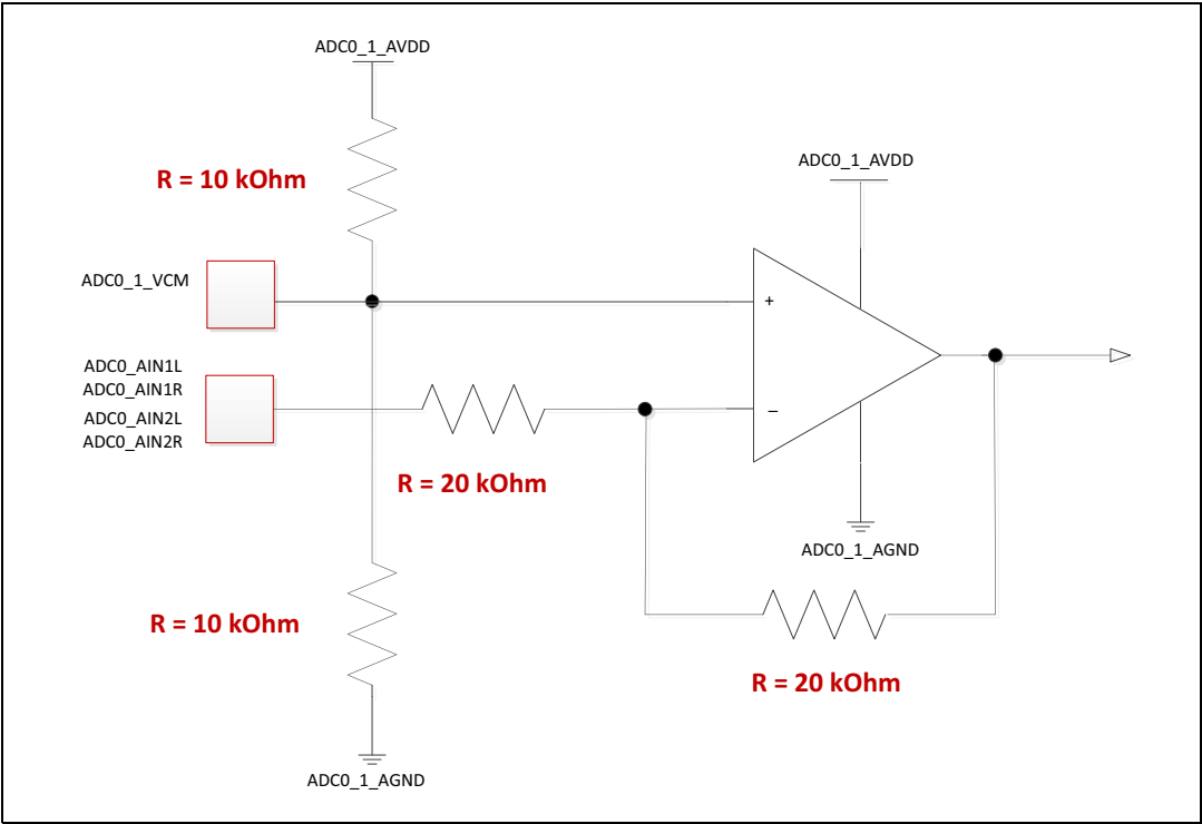
Figure 7. Audio ADC input equivalent circuit
