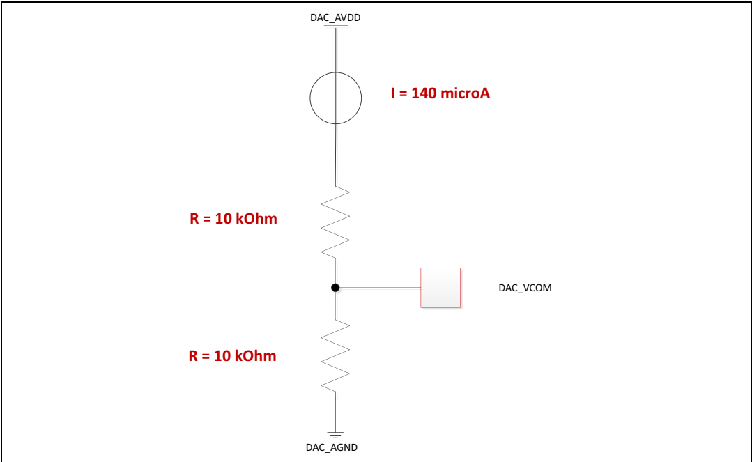
Figure 10. DAC VCOM equivalent circuit
