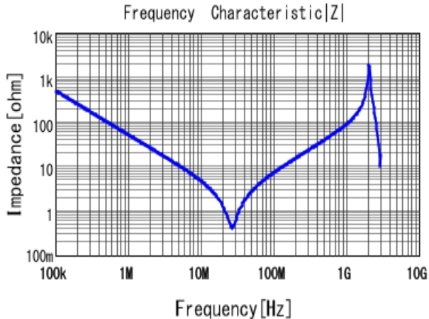
■ DE1E3KX332MN4AP01F |Z| DC0V, 20degC
