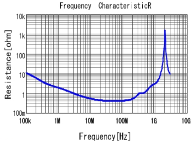
■ DE1E3KX332MN4AP01F R DC0V, 20degC
