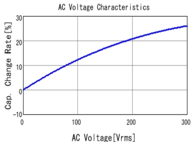
■ DE1E3KX332MN4AP01F C-AC Voltage capchange, DC0V, 20.0
