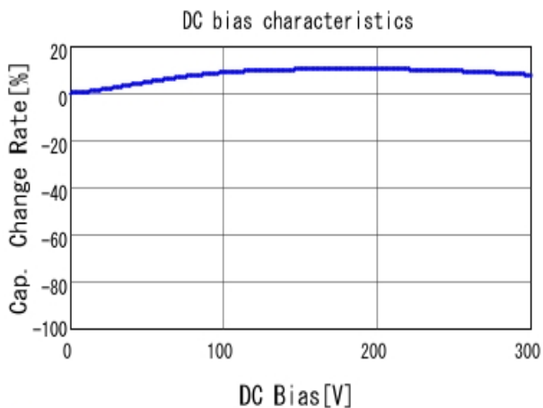
■ DE1E3KX332MN4AP01F C-DC bias capchange, 20.0degC, AC1
