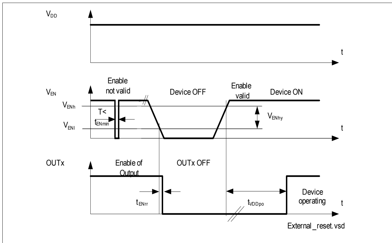
Figure 7 Timing
