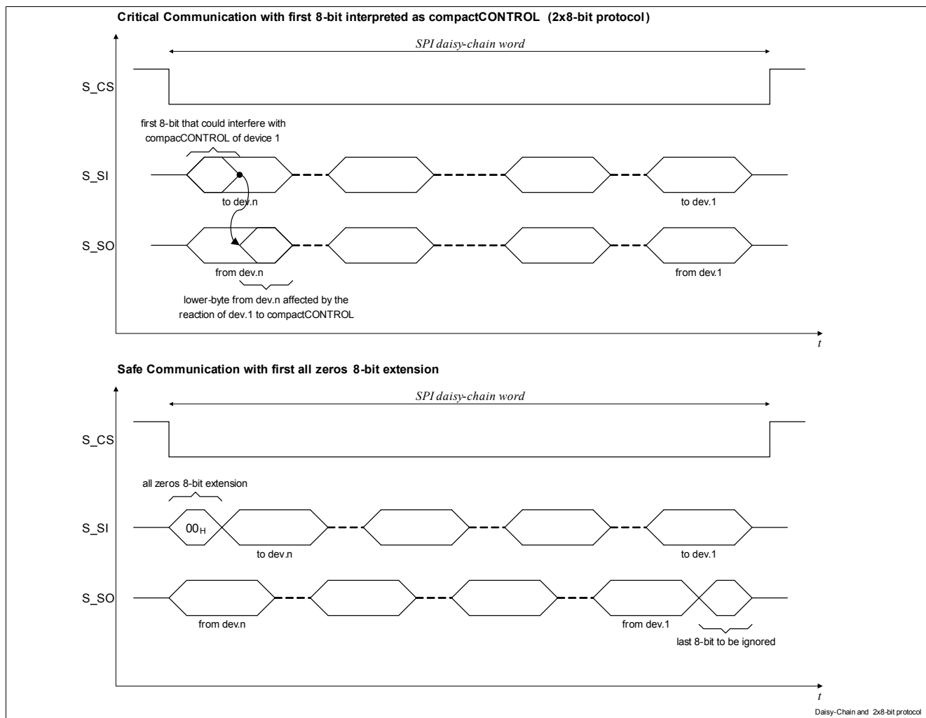
Figure 31 Daisy-Chain and 2x8-bit protocol
